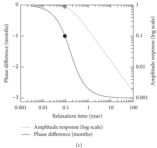
FIGURE 3: Relaxation RC system. (a) Equivalent circuit. (b) Temporal response. (c) Phase difference (dark curves) and amplitude (gray curve, log scale) of response. Note that the maximum phase difference is 3 months. The dot represents the radiation-temperature system, where the warmest (coldest) day is about one month after the “longest” (“shortest”) day, indicating a relaxation time of about 0.1 year (1.2 months).
