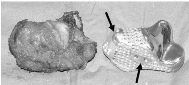
Fig. 4 3DP calcaneal prosthesis to replace a totally removed calcaneum. 33
