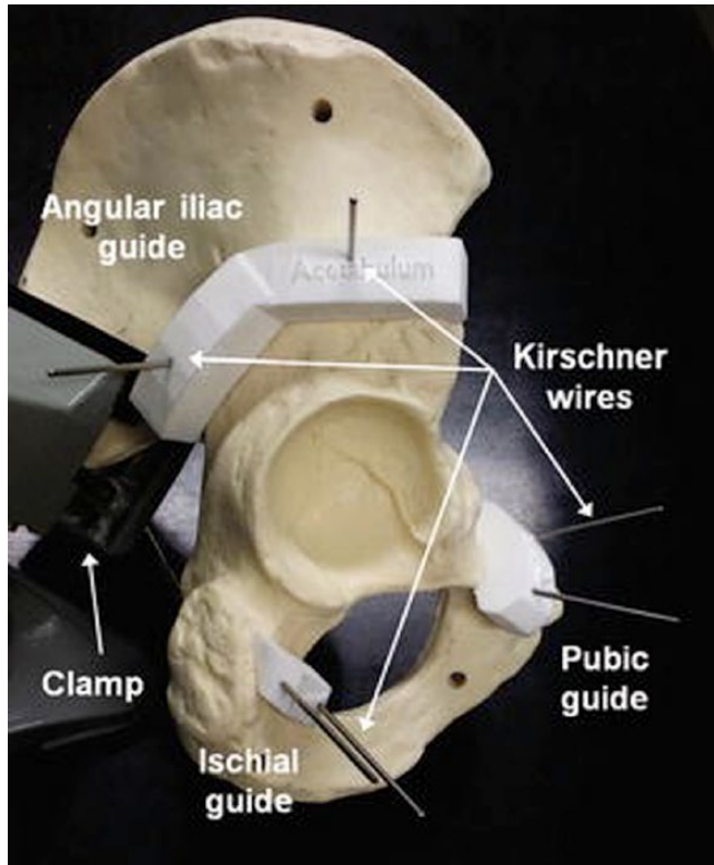
Fig. 6 PS surgical guides mounted on a PS pelvic bone model. 47
