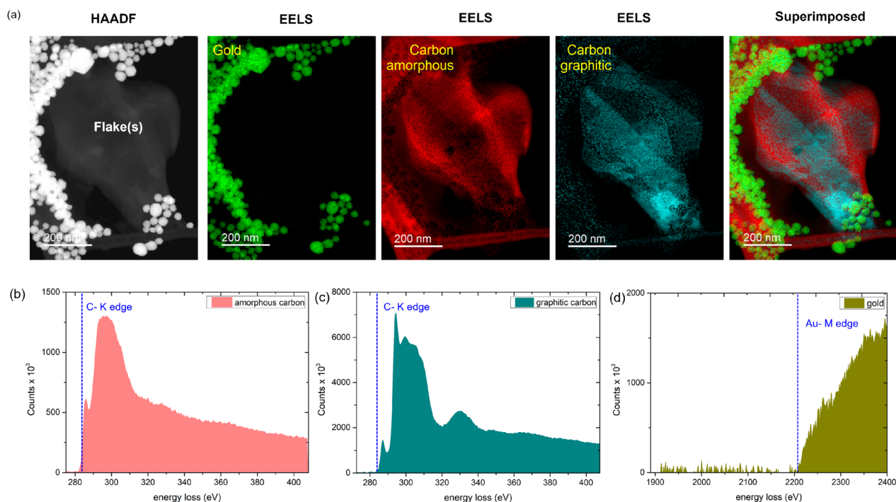
Fig. 4 (a) HAADF image of a collection of graphene flakes with gold nanoparticles (AuNPs), and corresponding EELS elemental mapping signatures of AuNPs, amorphous carbon, and graphitic carbon. The final image is the superimposed elemental map of all the elements. The color assignment is arbitrary. (b)–(d) Representative EELS spectra for amorphous carbon, graphitic carbon, and gold, respectively, obtained at their respective locations in the image. The C-K edge at 284 eV and Au-M edge at 2206 eV are highlighted.
