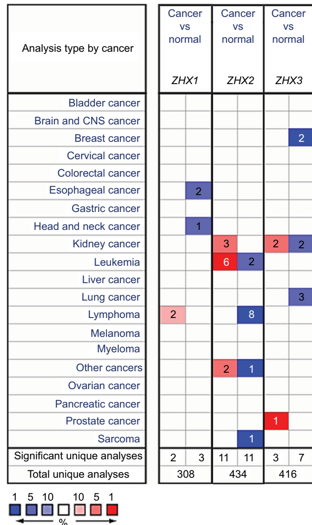
Figure 1 Transcriptional levels of ZHX family members in different cancer types and cancer cell lines. Notes: This graphic was obtained from Oncomine ( www.oncomine.org ) indicates the numbers of datasets with significant overexpression (red) or downexpression (blue) of ZHXs at transcriptional levels in cancer tissues compared with those in corresponding normal tissues. Cell color was determined by the best gene rank percentile for the analyses within the cell, and the gene rank was analyzed by the percentile of target genes in the top of all genes measured in each research. Abbreviation: CNS, central nervous system.
