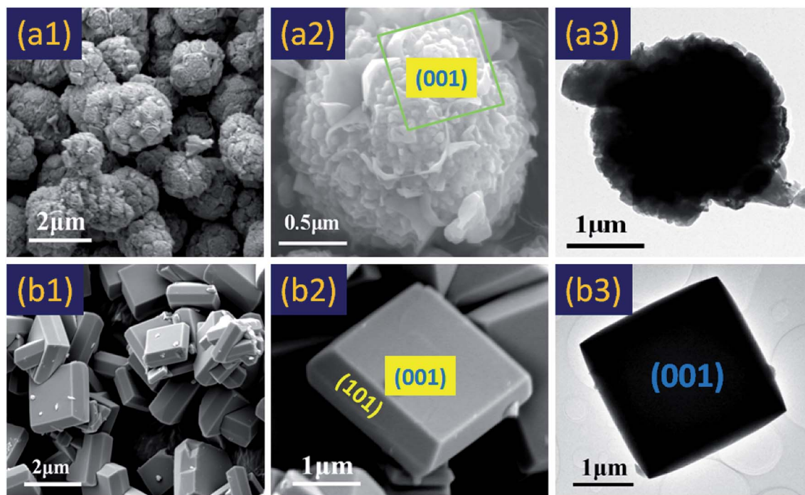
Fig. 1 Microstructure and morphology of anatase TiO 2 crystals. (a1), (a2) and (a3), SEM and TEM images of typical spherical TiO 2 polycrystalline particles (without HF). (b1), (b2) and (b3), SEM and TEM images of typical anatase TiO 2 single crystals (with HF).
