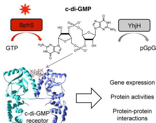
Figure 5. Regulation of diverse biological activities via the NIRW light-activated c -di-GMP module. NIRW light-controlled synthetic c -di-GMP module can be linked to output modules via c -di-GMP receptor proteins and RNA to regulate various biological activities. The structure of a VpsT receptor (PDB ID, 3klo) is shown as an example.
