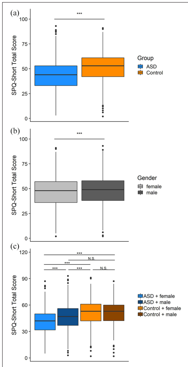
Figure 2. SPQ-Short scores distributions. Figure 2(a) shows distribution by group and (b) shows the distribution by gender; (c) shows distributions per gender and group. Horizontal black lines indicate medians, upper and lower bounds correspond to 75th and 25th percentiles, respectively. Whiskers extend until 1.5 the interquartile range, black dots indicate outliers beyond this.
