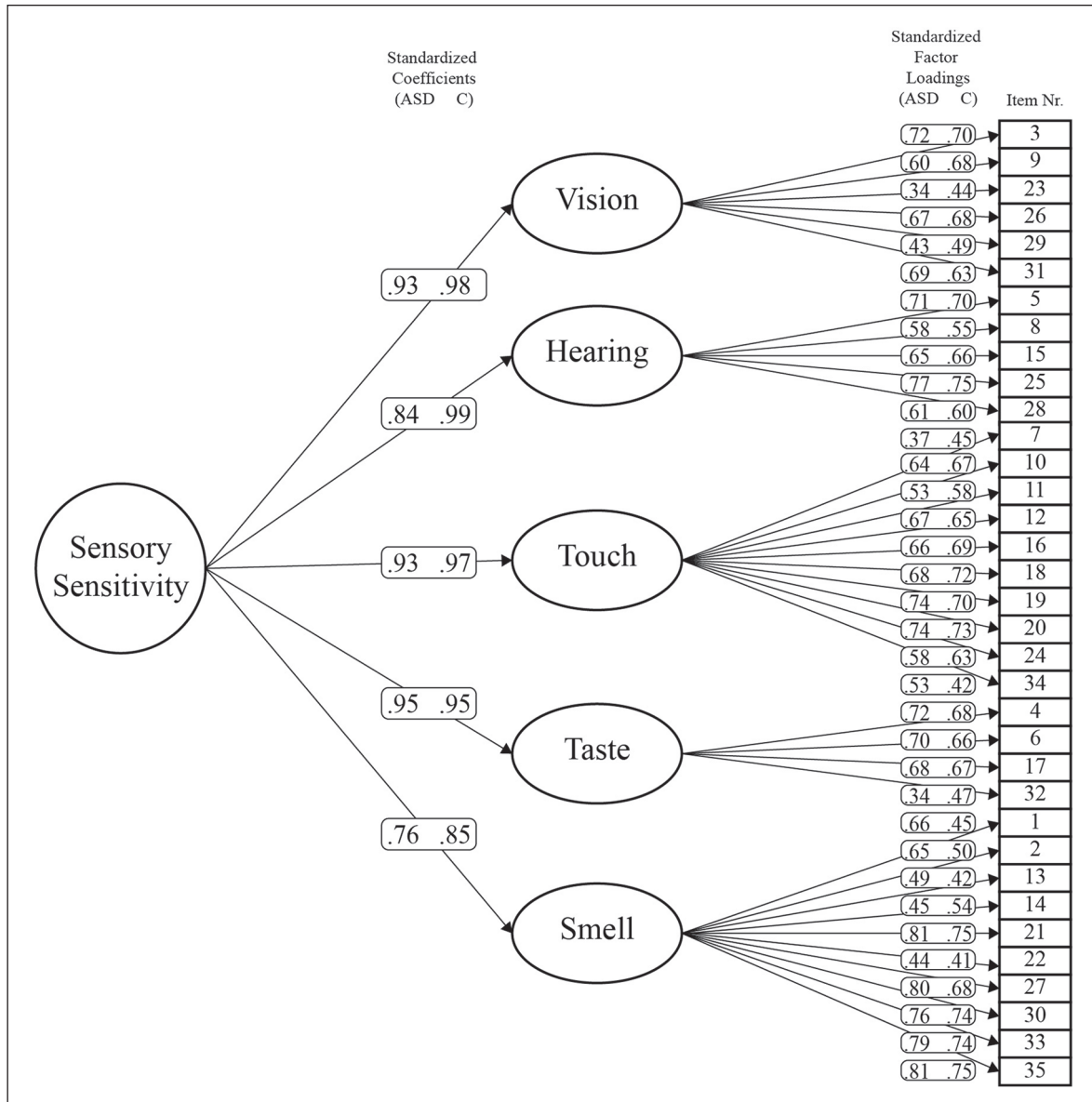
Figure 1. Hierarchical factor model of the SPQ-Short. Depicted are standardized factor loadings per group (ASD left, control right). Items (squares) first load onto their respective modality specific factor. All modality specific factors load in turn onto the higher-order modality-independent factor.
