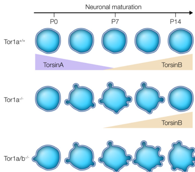
Figure 2. TorsinB dictates developmental vulnerability to torsinA LOF-related NE blebbing. Abnormal NE blebbing occurs during a developmental window when torsinB levels are low. Blebs resolve as torsinB levels rise during maturation. Simultaneous deletion of torsinA and torsinB prevents bleb resolution, highlighting how the torsinB expression level dictates susceptibility to torsinA LOF. Illustrated by Rachel Davidowitz.
