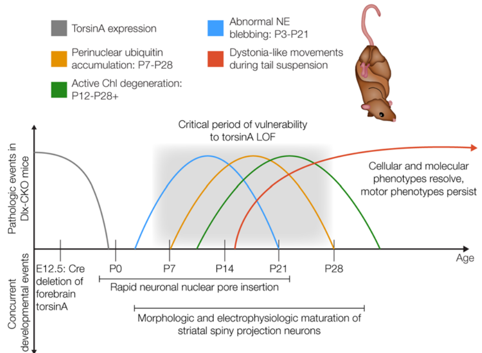
Figure 1. A neurodevelopmental model of DYT1 pathogenesis. Timeline of molecular, cellular, and behavioral events in Dix-CKO mice, as well as concurrent and potentially related developmental processes (109, 140). Molecular and cellular phenotypes emerge throughout a discrete period of vulnerability to torsinA impairment during early postnatal CNS maturation. These phenotypes rapidly disappear or stabilize, but motor dysfunction persists for life. This model highlights that initial torsinA-linked molecular events can lead to permanent circuit dysfunction delinked from the initial genetic insult. The sources for the phenotypes defined are as follows: NE blebbing (84), perinuclear ubiquitin accumulation, cholinergic interneuron (ChI) degeneration, and motor dysfunction (94). Illustrated by Rachel Davidowitz.
