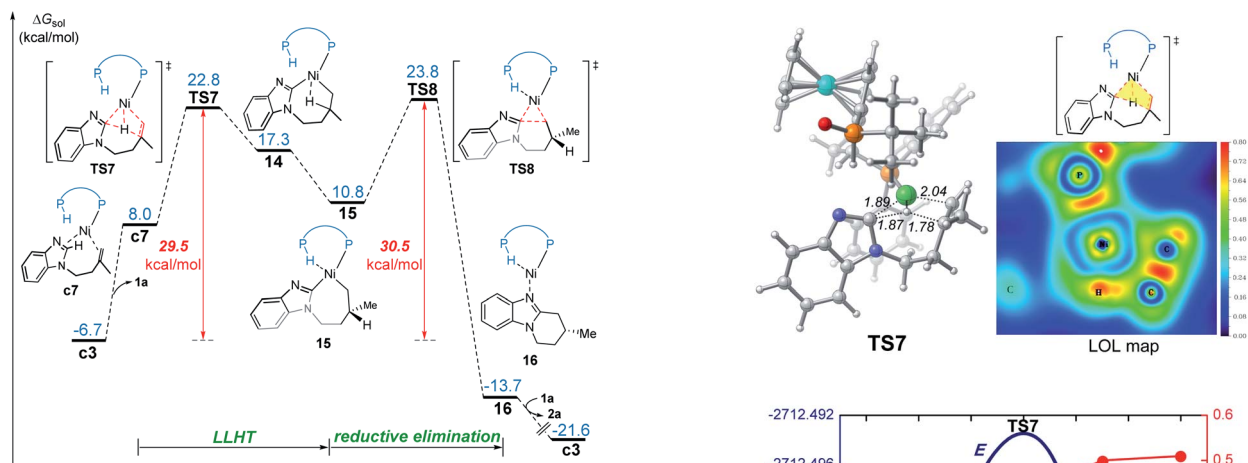
Fig. 6 Free energy profile for nickel(0)-promoted hydroarylation via the LLHT mechanism.
