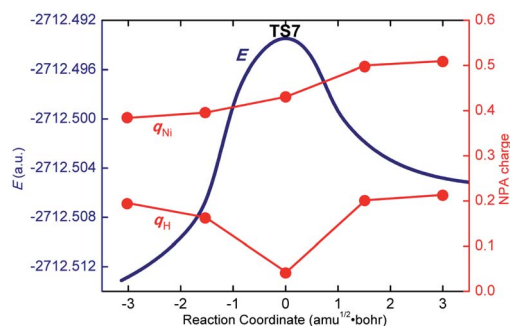
Fig. 7 Optimized structure of the LLHT transition state TS7 with selected bond distances in Å, the LOL map, and the electronic energies ( E ) and NPA charges ( q ) along the intrinsic reaction coordinates.
