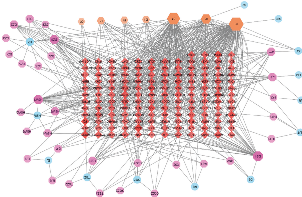
FIGURE 3: Compound-potential target network. Each blue ellipse represents a herb in ZSYT, and the pink octagons represent active compounds. The red diamonds represent the potential targets, and the orange hexagons at the bottom represent common active compounds. The size and transparency of each node are proportional to the target degree in the network.
