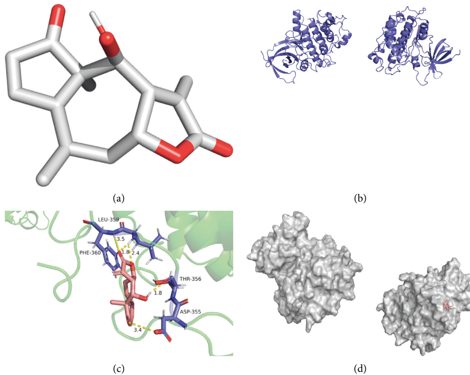
FIGURE 7: GSK3B helenalin molecular docking. 3D structures of (a) helenalin and (b) GSK3B. (c) Molecular docking simulation and (d) display protein surface of molecular docking simulation.
