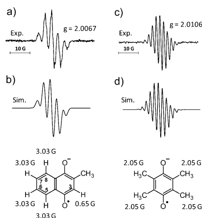
Figure 2. X-band EPR spectra at around 290 K. a) Menadione radical anion ( \text{M}^{\cdot-} ) generated by the reduction of menadione (1 mM) by NADH (0.5 mM) catalyzed by complex 1 or 3 (160 \mu\text{M} ) in phosphate buffer (pH 7.2, 9 h). b) Simulated \text{M}^{\cdot-} EPR spectrum with hyperfine coupling constants. c) Durosemiquinone radical anion ( \text{D}^{\cdot-} ) generated by reduction of duroquinone (2 mM) by NADH (1 mM) catalyzed by complex 1 or 3 (330 \mu\text{M} ) in phosphate buffer (pH 7.2, 10 h). d) Simulated \text{D}^{\cdot-} EPR spectrum with hyperfine coupling constants.
