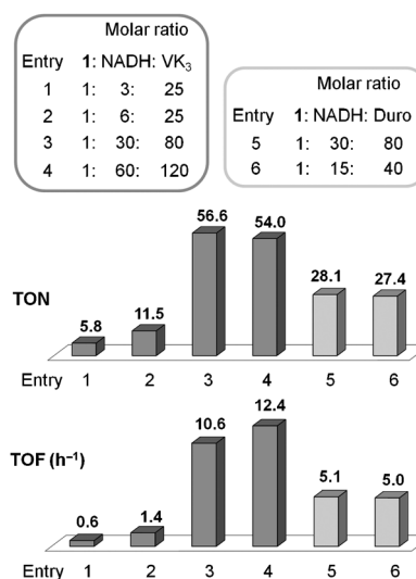
Figure 3. Reduction of menadione (VK 3 , entries 1–4) and duroquinone (Duro, entries 5 and 6) by NADH catalyzed by complex 1 (80 \mu\text{M} ).
