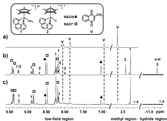
Figure 1. ^1\text{H} NMR spectra showing the formation of complex 2 [(\eta^5\text{-C}_5\text{Me}_5)\text{Ir}(\text{phen})(\text{H})]^+ and its reaction with menadione in [\text{D}_4]\text{MeOD}/\text{H}_2\text{O} (1:9) at 298 K. a) Menadione alone. b) Formation of hydrido complex 2 from reaction of [(\eta^5\text{-C}_5\text{Me}_5)\text{Ir}(\text{phen})(\text{H}_2\text{O})]^{2+} ( 1 ; 1 mM) with NADH (2 mM). c) Disappearance of signals of hydride 2 and broadening of signals of menadione 10 min after addition of menadione (1 mM) to mixture in (b).
