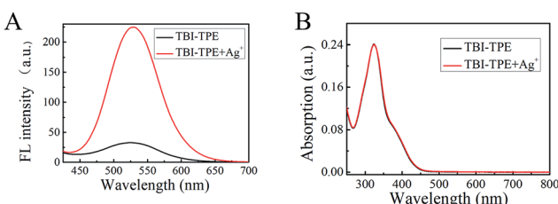
Fig. 2 (A) Fluorescence spectra. (B) UV absorption spectra of TBI-TPE (4 \mu\text{M} ) in \text{CH}_3\text{OH} in the presence of \text{Ag}^+ (4 \mu\text{M} ), E_x = 370 nm.
