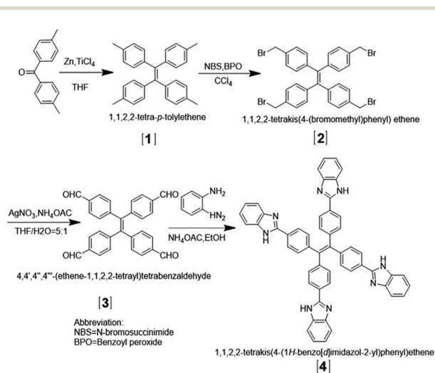
Scheme 1 Synthetic route to new 1,1,2,2-tetrakis(4-(1 H -benzo[ d ]imidazole-2-yl)phenyl)ethene molecules, TBI-TPE.
