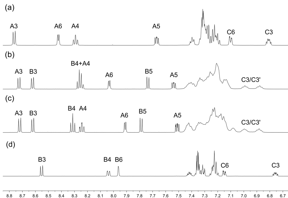
Figure 1. ^1\text{H} -NMR spectra (aromatic regions, 500 MHz, acetone- d_6 , 298 K) of (a) [\text{Cu}(\text{BIPHEP})(\text{bpy})][\text{PF}_6] , (b) [\text{Cu}(\text{BIPHEP})(6\text{-Mebpy})][\text{PF}_6] , (c) [\text{Cu}(\text{BIPHEP})(6\text{-Etbp})][\text{PF}_6] and (d) [\text{Cu}(\text{BIPHEP})(5,5'\text{-Me}_2\text{bpy})][\text{PF}_6] .
