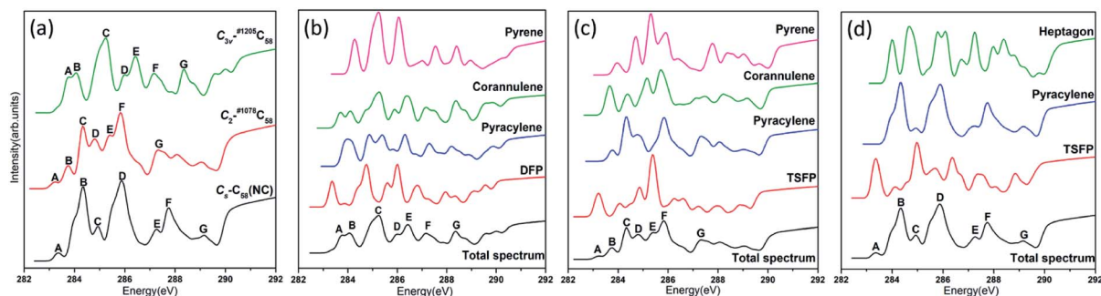
Fig. 5 Calculated (a) total NEXAFS spectra of the three C_{58} isomers as well as type-specific contributions for (b) C_{3v} - \#1205C_{58} , (c) C_{2-} - \#1078C_{58} and (d) C_s - C_{58} (NC). Each total spectrum is obtained by weighted (according to their relative abundance) summation of all type-specific spectra.
