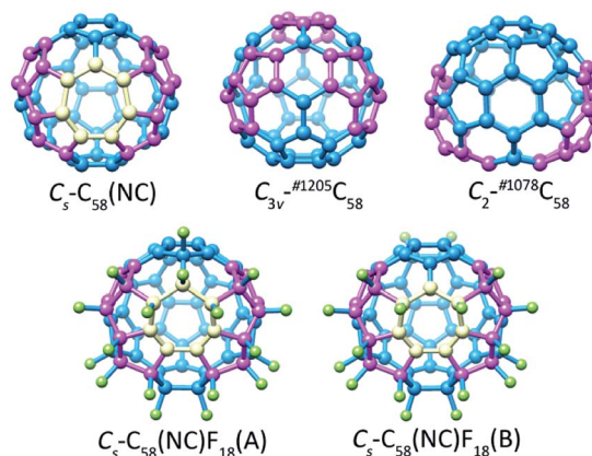
Fig. 1 Optimized structures of the non-IPR isomers C_{3v}^{-\#1205}C_{58} and C_{2}^{-\#1078}C_{58} , as well as the non-classical isomer C_s-C_{58}(NC) with its fluorinated derivatives C_s-C_{58}(NC)F_{18}(A) and C_s-C_{58}(NC)F_{18}(B) .
