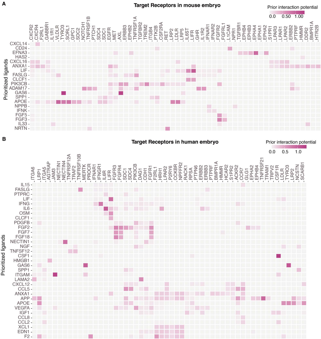
Figure 4. Potential interactions between receptive epithelium and implantation competent embryos. The prioritized ligands in receptive epithelium and their target signaling pathways in competent embryos in mouse (A) and human (B).
