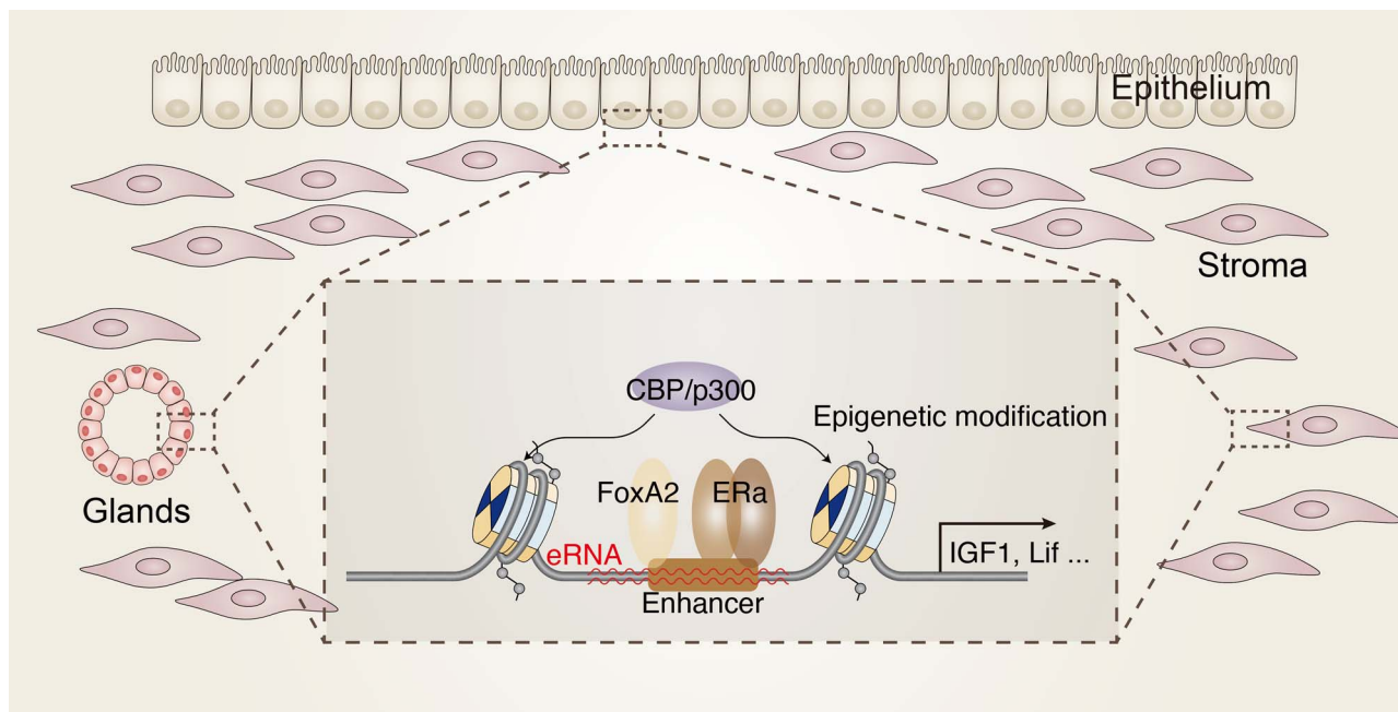
Figure 2. The genomic transcriptional activation of ER in uterus.
