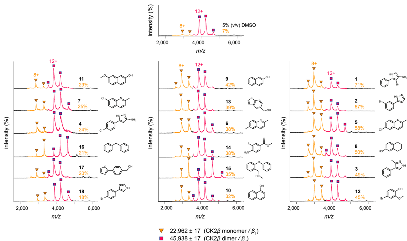
Figure 3. Native mass spectra of 16 \mu\text{M} CK2 \beta , acquired in 0.5 M ammonium acetate pH 8.0, in the presence of validated thermally destabilizing fragments (2 mM). The percentage of CK2 \beta monomerization induced by a fragment is indicated in orange text below the compound number. Charge states are colored and indicated with symbols. The observed mass and identity of each species are indicated beside the symbols. Only one charge state of each species is indicated in the spectra.
