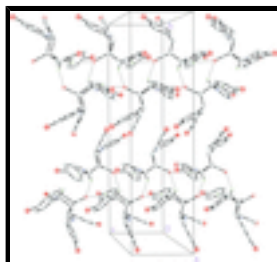
Fig. 2. The crystal packing of the title compound, showing the extended one-dimensional chains linked along the c axis. H atoms not involved in the intermolecular interactions (dashed lines) have been omitted for clarity. Only the major components are shown.
