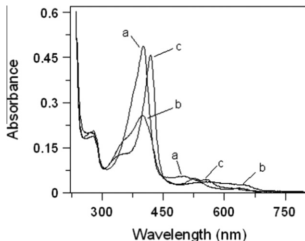
Fig. 5. Absorption spectra of Euphorbia peroxidase . (a) ELP native enzyme (3.7 \mu\text{M} ); (b) Compound I is formed after addition of equimolar amount of hydrogen peroxide to the native enzyme. (c) Compound II is formed after addition of approximately 3.7 nmol NO to Compound I. Addition of another amount of NO reduced Compound II to the native enzyme. Buffer 100 mM Tris-HCl, pH 7.0.
