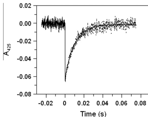
Fig. 4. Laser photolysis of ELP-Fe III with NO. Time course of NO rebinding to ferric ELP after photolysis. Experimental conditions: 8 \mu\text{M} ELP, buffer 100 mM Tris-HCl, pH 7.0, T = 25^\circ\text{C} , observation wavelength 425 nm.
