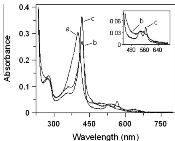
Fig. 9. Absorption spectra of Euphorbia peroxidase in the presence of CN - . (a) Native peroxidase (2.4 μM) in anaerobic conditions; (b) as (a) in the presence of 15 μM CN - . (c) Addition of an excess of NO to (b). Readmission of oxygen causes the gradual formation of the native enzyme. Inset: expanded absorption visible spectrum showing the differences between (b) and (c).
