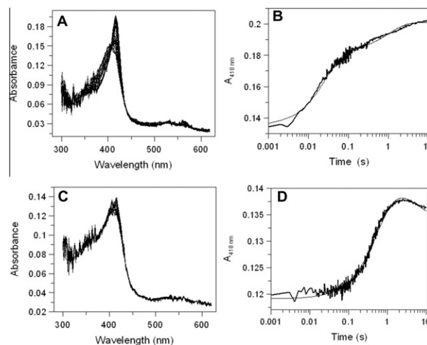
Fig. 8. Time-resolved absorbance spectra recorded after mixing Compound I with excess NO. Panel A: absorbance spectra recorded after mixing a 3.7 \mu M solution of the Compound I of ELP (obtained by addition to the native enzyme of 3 \mu M H_2O_2 ) with 25 \mu M NO, in 100 mM Tris-HCl buffer, pH 7.0, T = 25^\circ C , in the absence of calcium ions. Panel B: time course of the experiment in Panel A at 418 nm; the continuous line is the result of fitting the data to two sequential exponential decays (see text). Panel C: experiment as in Panel A, but in the presence of 10 mM CaCl_2 . Panel D: time course of the experiment in Panel C at 418 nm.
