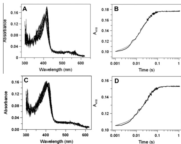
Fig. 3. Time-resolved absorbance spectra recorded after combination of ELP-Fe III with NO. Panel A: time resolved spectra recorded upon mixing 2.3 \mu\text{M} ferric ELP with 40 \mu\text{M} NO (concentrations before mixing). Buffer 100 mM Tris-HCl, pH 7.0; T = 25^\circ\text{C} . Panel B: time course at 418 nm extracted from the data reported in Panel A. Panel C: as in Panel A but in the presence of 10 mM \text{CaCl}_2 . Panel D: time course at 418 nm extracted from the data reported in Panel C.
