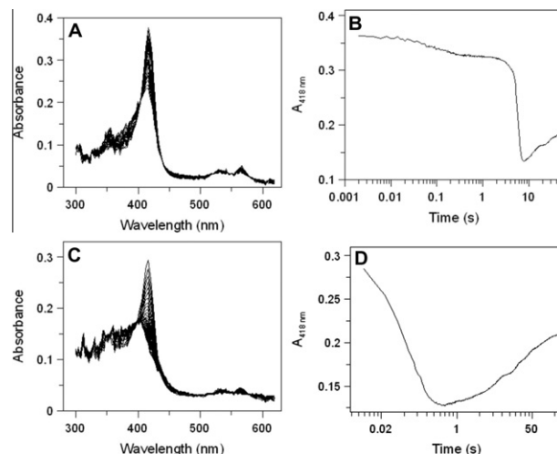
Fig. 7. Time-resolved absorbance spectra recorded after mixing ELP- Fe^{III} -NO with H_2O_2 . Panel A: Absorbance spectra recorded after mixing a 3.7 \mu M solution of ELP, in 100 mM Tris-HCl buffer, pH 7.0, T = 25^\circ C , containing 100 \mu M NO with a 200 \mu M solution of H_2O_2 , in the absence of calcium ions. Panel B: time course of the experiment in Panel A at 418 nm; notice that release of bound NO is required before the steady state starts. The end of the steady state is marked by the appearance of Compound I, coupled to a very significant decrease of absorbance. The final absorbance increase is presumably due to the partial conversion of Compound I to Compound II caused by H_2O_2 itself. Panel C: experiment as in Panel A, but in the presence of 10 mM CaCl_2 . Panel D: time course of the experiment as in Panel C at 418 nm. The much faster appearance of Compound I in the presence of calcium (compared with Panel B) is due to the fact that under these experimental conditions the reaction of ELP with H_2O_2 is much faster and thus the steady state mixture is dominated by Compound I, which would be virtually absent in the absence of the cation.
