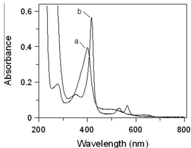
Fig. 2. Electronic absorption spectral change upon NO binding to the ELP– \text{Fe}^{\text{III}} . (a) ELP native enzyme (3.1 \mu\text{M} ) in anaerobic conditions and (b) after addition of NO in excess. Buffer 100 mM Tris–HCl, pH 7.0.
