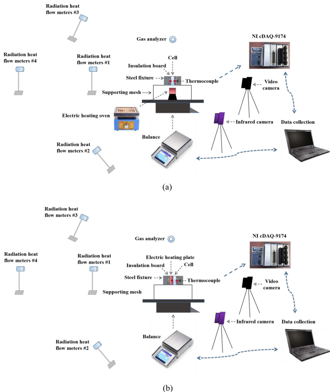
Fig. 1 Schematic of the experimental setup: (a) electric heating oven; (b) electric heating plate.
