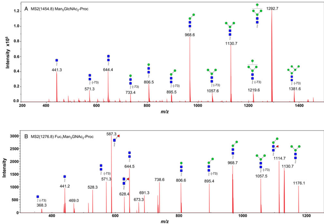
Fig. 7. Positive-ion MS/MS spectra of \text{Man}_5\text{GlcNAc}_2\text{-Pro} (A) and \text{Fuc}_1\text{Man}_3\text{GlcNAc}_2\text{-Pro} (B) from O. ochengi GST1. (-73) refers to [M + H]^+ ions that have lost terminal diethylamine from the procainamide tag during the collision (Kozak et al. , 2015). Blue squares, N -acetylglucosamine residues; green circles, mannose residues; red triangles, fucose residues; Proc, procainamide tag.
