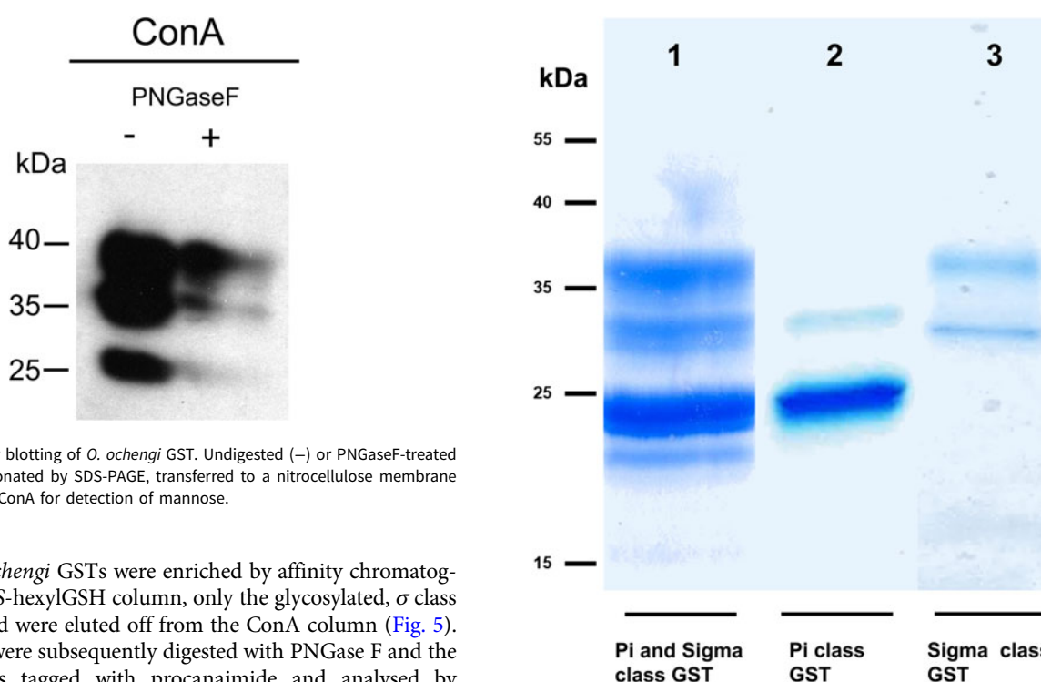
Fig. 5. SDS PAGE gel showing O. ochengi glutathione transferases (GSTs), resolved via S -hexylGSH-affinity and ConA-lectin-affinity chromatography. All bands shown in the SDS PAGE image were glutathione transferases (GSTs) of \pi and \sigma classes, purified and identified via tandem mass spectrometry. Lane 1, GSTs of \pi and \sigma classes resolved from cytosolic extracts eluted from an S -hexylGSH-affinity column. Lane 2, S -hexylGSH-affinity GSTs of the \pi class that does not bind to the ConA-lectin-affinity column. Lane 3, ConA-lectin-binding \sigma class GSTs that also bind the S -hexylGSH-affinity column.
