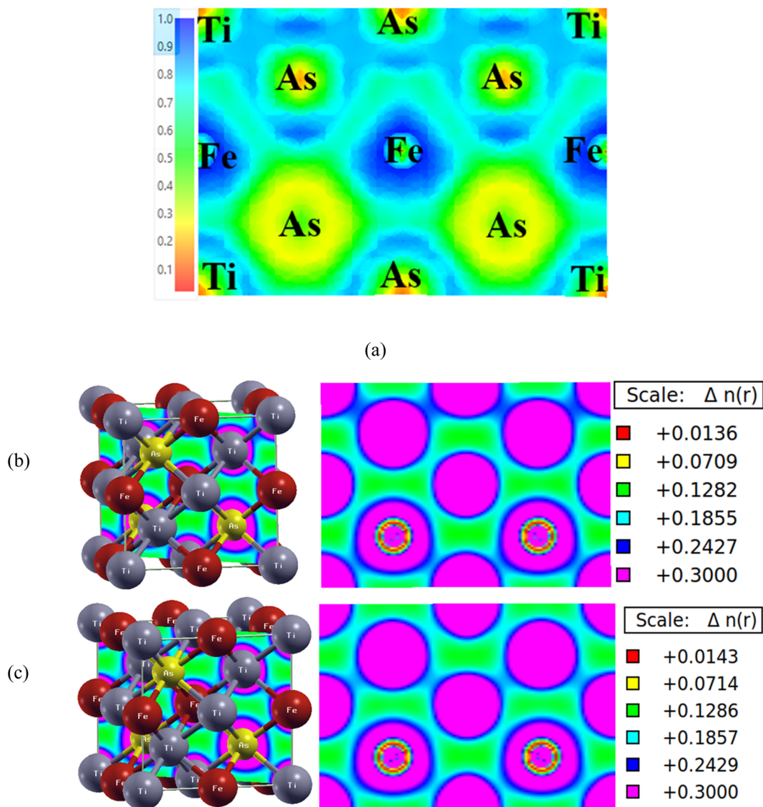
Fig. 6 (a) Electron localization function (ELF) along the 110 plane and plot of charge density distribution along the (110) plane of \text{Ti}_2\text{FeAs} compound for (b) spin up and (c) spin down, respectively.
