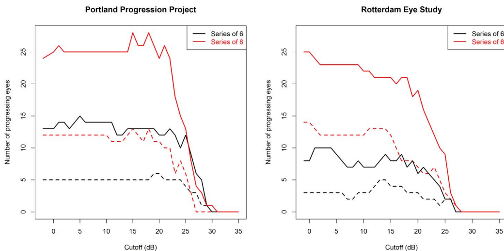
FIGURE 3. The number of eyes flagged as progressing by pointwise linear regression are shown after censoring sensitivities below some cutoff CdB to set them equal to CdB. Solid lines: An eye was labeled progressing if three or more locations were progressing (slope worse than -1 dB/year, with a significance of P < 1\% ). Dashed lines: An eye was labeled progressing if three or more neighboring locations were progressing. Analysis was performed using the last six ( black ) or the last eight ( red ) visual fields in the series for each eye.
