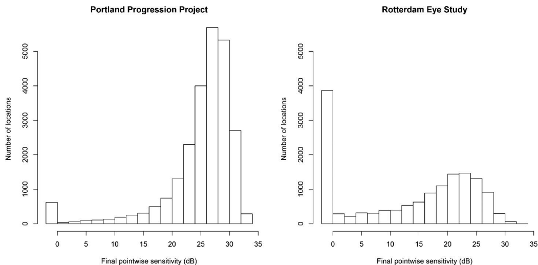
FIGURE 1. Histograms of the final pointwise sensitivities in each series for the two datasets.
