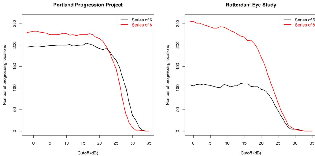
FIGURE 2. The number of locations flagged as progressing by pointwise linear regression are shown after censoring sensitivities below some cutoff CdB to set them equal to CdB. A progressing location was defined as one whose sensitivity decreased at a rate worse than -1 dB/y, with a significance of P < 1\% . Analysis was performed using the last six ( black ) or the last eight ( red ) visual fields in the series for each eye.
