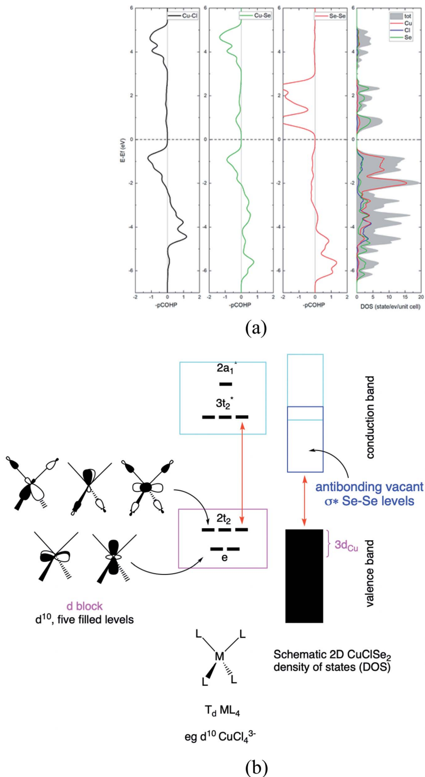
Fig. 6 (a) Calculated COHP curves and DOS for two-dimensional P2_1 \text{CuClSe}_2 . (b) Schematic of the 2D P2_1 \text{CuClSe}_2 density of states. The metal MO levels of the isolated d^{10} tetrahedral \text{ML}_4 fragment are displayed on the left.
