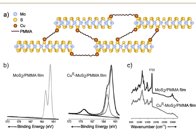
Fig. 10 (a) Scheme of the Cu II -MoS 2 /PMMA structure. On the bottom part, (b) S 2p core level XPS spectra of the Cu-free and Cu-coordinated MoS 2 /PMMA films and (c) IR of the two different species. Adapted from ref. 94, Copyright 2013, Wiley-VCH.
