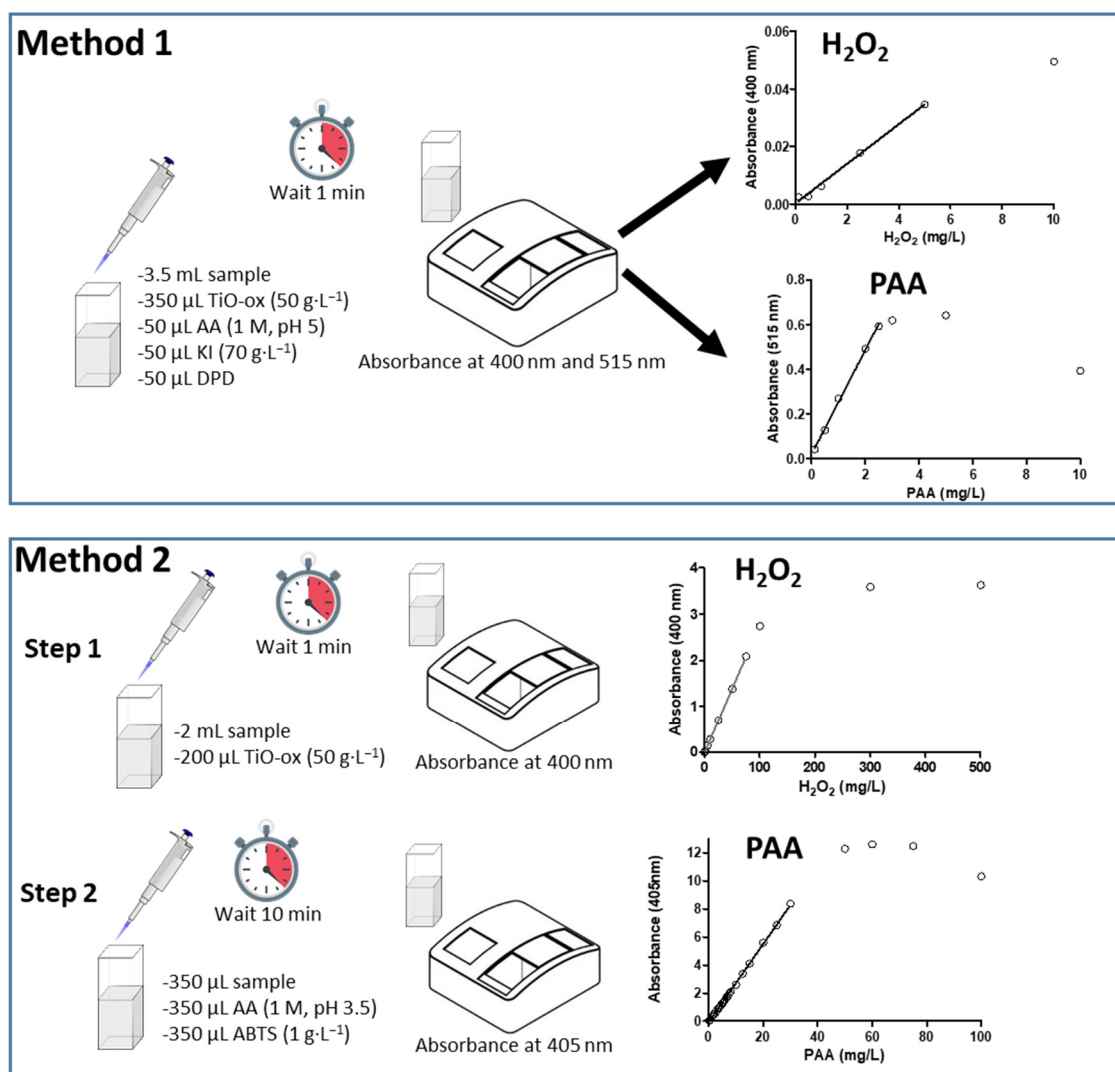
Figure 1. Schematic diagram showing the steps of the two methods used for quantification of peracetic acid (PAA) and hydrogen peroxide ( \text{H}_2\text{O}_2 ): (TiO-Ox: titanium oxide oxalate; AA: Acetic acid; KI: potassium iodide; DPD: N,N -dimethyl- p -phenylenediamine; ABTS: 2,2'-azino-bis(3-ethylbenzothiazoline-6-sulphonic acid)).
