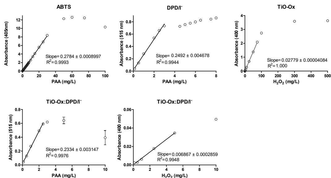
Figure 4. Calibration curve of PAA and H 2 O 2 using ABTS, DPD/I - , TiO-Ox:DPD/I - and TiO-Ox as color reagents, respectively. Error bars indicating standard deviation ( n = 3 ) are smaller than the symbol representing the averages for most concentrations. Note: different scales on the primary axes.
