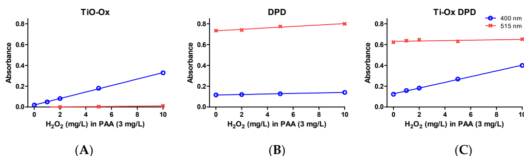
Figure 3. Absorbance of oxidized colorimetric reagents; absorbance of TiO-Ox obtained by oxidation with 0, 1, 2, 5 and 10 \text{ mg}\cdot\text{L}^{-1} \text{H}_2\text{O}_2 spiked in 3 \text{ mg}\cdot\text{L}^{-1} PAA (A); absorbance of \text{DPD}^+ obtained by oxidation with 0, 1, 2, 5 and 10 \text{ mg}\cdot\text{L}^{-1} \text{H}_2\text{O}_2 spiked in 3 \text{ mg}\cdot\text{L}^{-1} PAA (B) and absorbance of TiO-Ox: \text{DPD}^+ obtained by oxidation with 0, 1, 2, 5 and 10 \text{ mg}\cdot\text{L}^{-1} \text{H}_2\text{O}_2 spiked in 3 \text{ mg}\cdot\text{L}^{-1} PAA (C). Absorbance were recorded at 400 nm and 515 nm. Error bars indicating standard deviation ( n = 3 ) were always smaller than the symbol representing the averages.
