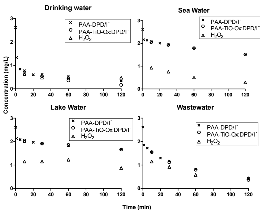
Figure 5. Concentration profiles of PAA and \text{H}_2\text{O}_2 in drinking water, sea water, lake water and wastewater effluent quantified using \text{DPD}/\text{I}^- and \text{TiO-Ox:DPD}/\text{I}^- colorimetric assay when spiked with 2.6 \text{ mg}\cdot\text{L}^{-1} PAA.
