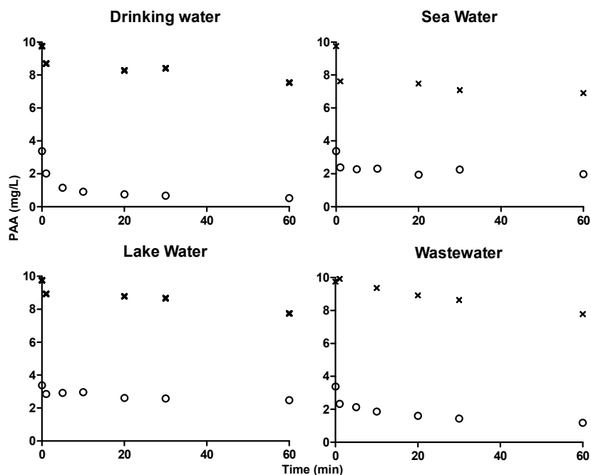
Figure 6. Concentration profiles of PAA in drinking water, seawater, lake water and wastewater quantified using ABTS colorimetric assay. 'x' symbol in the graphs represents the concentration profile of 10 \text{ mg}\cdot\text{L}^{-1} PAA and 'o' symbol in the graphs represents the concentration profile of 3 \text{ mg}\cdot\text{L}^{-1} PAA.
