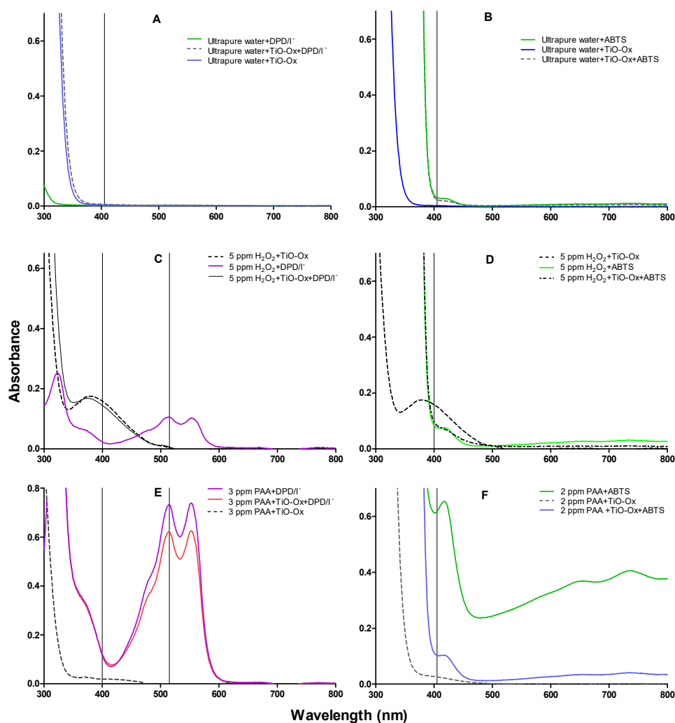
Figure 2. Absorption spectra of oxidized colorimetric reagents; (A) absorption spectra of DPD/I - , [TiO-Ox·DPD/I - ] and TiO-Ox mixed in ultrapure water to measure reagents background color and cross reactivity between the reagents, (B) absorption spectra of ABTS, [TiO-Ox·ABTS] and TiO-Ox mixed in ultrapure water to measure reagents background color and cross reactivity between the reagents, (C) absorption spectra of DPD + and [TiO-Ox·H 2 O 2 ] obtained by oxidation with 5 mg·L -1 H 2 O 2 , (D) absorption spectra of ABTS + , [TiO-Ox·H 2 O 2 ] and [TiO-Ox·ABTS + ·H 2 O 2 ] obtained by oxidation with 5 mg·L -1 H 2 O 2 , (E) absorption spectra of DPD + , and [TiO-Ox·DPD + ·PAA] obtained by oxidation with 3 mg·L -1 PAA. Spectra after color reaction with 3 mg·L -1 PAA, DPD/I - ; PAA, TiO-Ox, DPD/I - and PAA, TiO-Ox. All color reaction was maintained at pH 5 in presence of KI (70 g·L -1 ) and (F) absorption spectra of ABTS + , [TiO-Ox·PAA] and [TiO-Ox·ABTS + ·PAA] obtained by oxidation with 2 mg·L -1 PAA.
