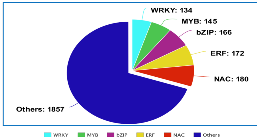
Figure 1. Pie chart showing the number of transcription factor (TF) genes in NAC, MYB, ERF, bZIP, WRKY, and other families in sorghum.
