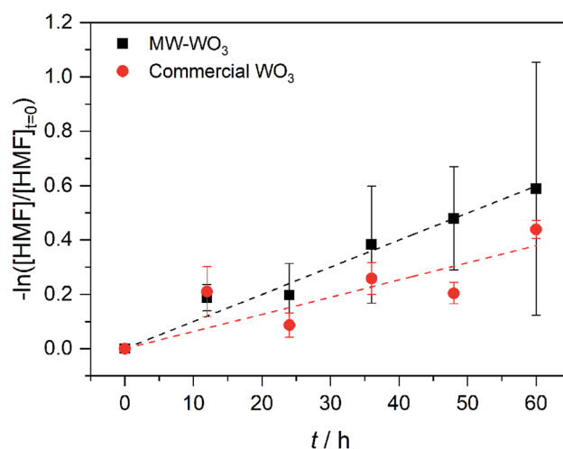
Fig. 7 First order rate plot for the photocatalytic oxidation of HMF on MW-WO 3 (black squares) and bulk WO 3 (red circles) using 460 nm blue LEDs.
