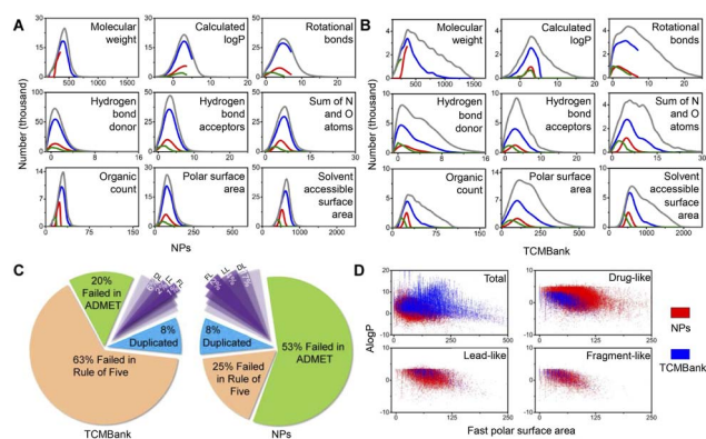
Fig. 13 Comparison with natural product databases. (A) In NPs' overall physical properties and (B) TCMBank overall physical properties, grey, blue, red, and green respectively represent all chemical compounds, drug-like, lead-like, and fragment-like. (C) Results of TCMBank and NPs going through ADMET and Rule of five selection. (D) ADMET distributions for TCMBank and NPs. NPs refer to natural product databases.
