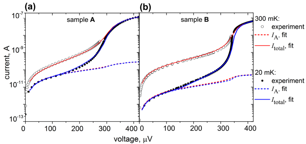
Figure 5. The fitting of IV-curves by HBE with Andreev current. (a) The sample A . (b) The sample B . The color legend from the right is valid for both (a,b) blue color is for 20 mK, red color is for 300 mK, dots are an experiment, solid curves are the total fitted current, the dashed curve shows Andreev current.
