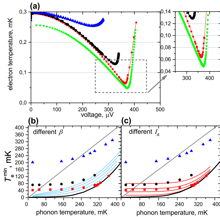
Figure 3. (a) Electron temperature obtained from HBE (2) versus voltage for three samples at T_{ph} = 300\text{mK} : triangles for the sample A, circles for the sample B, rectangles for the sample C. Diamonds are for the sample C at 256 mK. (b) Minimal electron temperature versus phonon temperature. Blue curves are calculated for various fixed \beta (0.0, 0.2, 0.4 and 0.6) and zero I_A . (c) Minimal electron temperature versus phonon temperature. Red curves are calculated for various I_A and zero \beta . I_A changes from 30 pA to 4 nA. Thick black solid curve is an ideal theory without Andreev current and without heat return. In addition, experimental points are given: triangles for the sample A, circles for the sample B, rectangles for the sample C.
