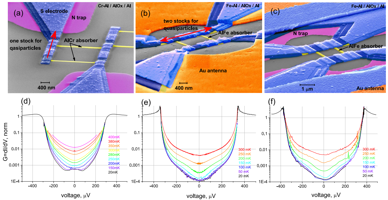
Figure 2. SEM images of the sample designs with one stock and normal metal traps for quasiparticles (a), with two stocks and without traps (b) and with two stocks and normal metal traps (c). Here the gold antennas are shown in orange, the superconductors in blue, the N traps in magenta, and the absorber in yellow, with a typical volume of its narrow part of 15 \text{ nm}^3 \times 80 \text{ nm}^3 \times 1000 \text{ nm}^3 . Red arrows in (a,b) show the possible directions for quasiparticles to move. In (a), there is only one direction, which results in the S electrode overheating. Plots on (d,e,f) are differential conductivities of the samples A, B, and C, at various temperatures, respectively. In (d), the presence of Andreev current I_A is evident below 150 mK as a slight peak at zero voltage. In (e,f), there is no visible sign of I_A down to 20 mK. Much better electron cooling is seen in (e,f) in comparison with (d).
