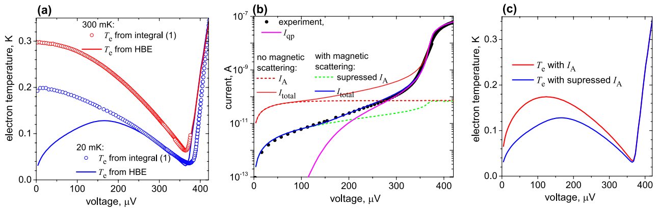
Figure 4. The fitting results for the sample C. (a) The electron temperature determined by two different methods: symbols are for using integral for quasiparticle tunneling (1), lines for using HBE (2) and (3), blue and red colors are for plate temperatures 20 mK and 300 mK, respectively. (b) Current–voltage characteristic at 20 mK. Dots represent an experiment, and magenta is quasiparticle current. The red solid curve shows the total current if Andreev current (dashed red curve) is not suppressed. The blue solid curve is the total current with suppressed Andreev current (dashed green). (c) Electron temperature versus voltage at T_{ph} = 20\text{mK} in case of suppressed and non-suppressed Andreev current.
