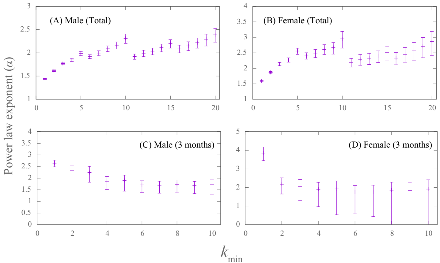
Fig 3. The estimated values of the power-law exponents ( \alpha ) in a function of k_{\min} . (A) and (B) are cumulative (total) sexual partners for males and females, respectively. (C) and (D) represent males and females in the previous three months, respectively. The error bars represent the 95% confidence intervals evaluated by the nonparametric (percentile) bootstrap method.
