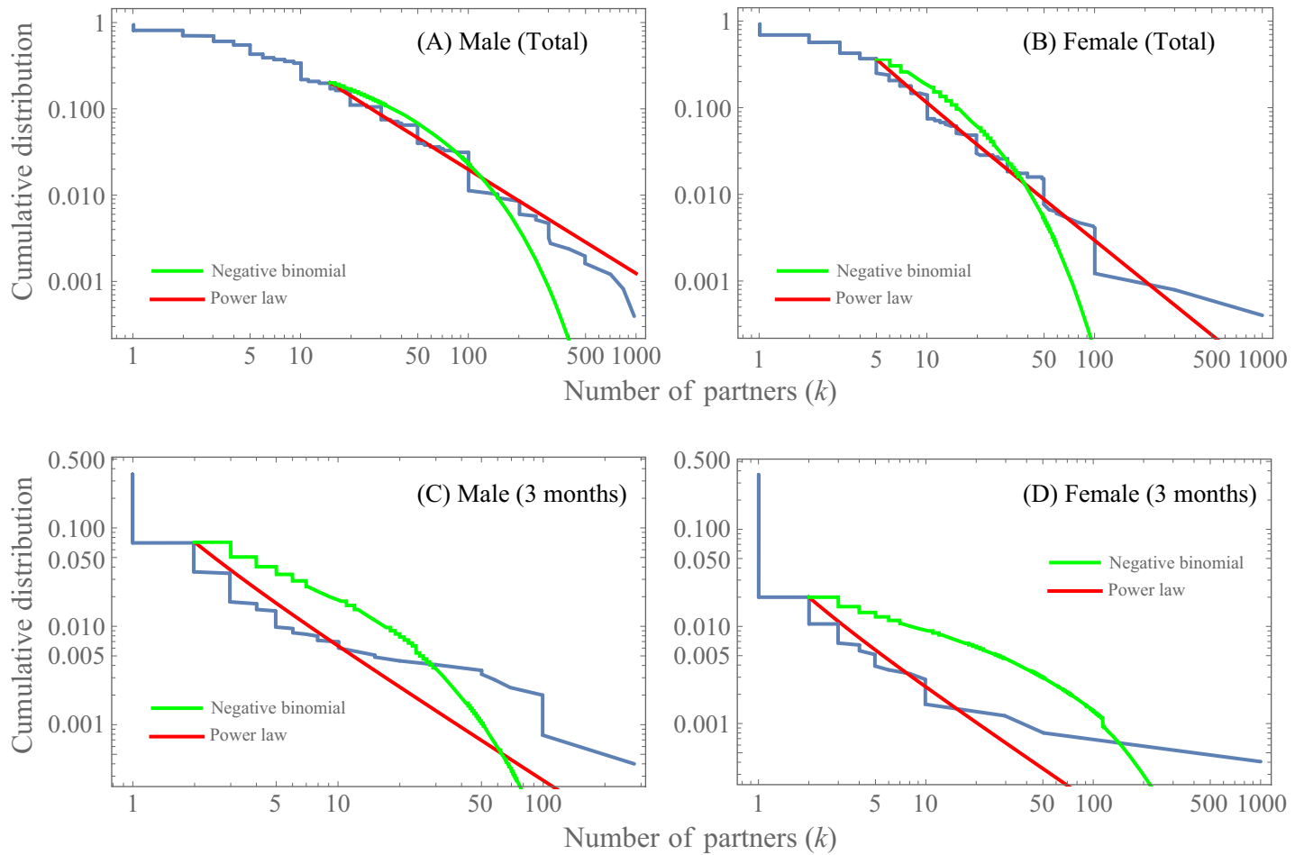
Fig 1. The cumulative distributions of the number of sexual partners. The cumulative distributions for the number of cumulative (total) sexual partners for (A) males and (B) females, respectively. (C) and (D) show the cumulative distributions of the number of sexual partners for males and females in the previous three months, respectively. The red and green curves represent the maximum likelihood fitting of the power-law distribution and the negative binomial distribution, respectively. Here, we use k_{min} as shown in Table 1. The estimated value and confidence interval of the power-law exponent are given in Table 1.
