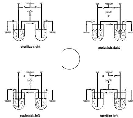
Figure 1 Operation cycle of an alternating tandem chemostat.
