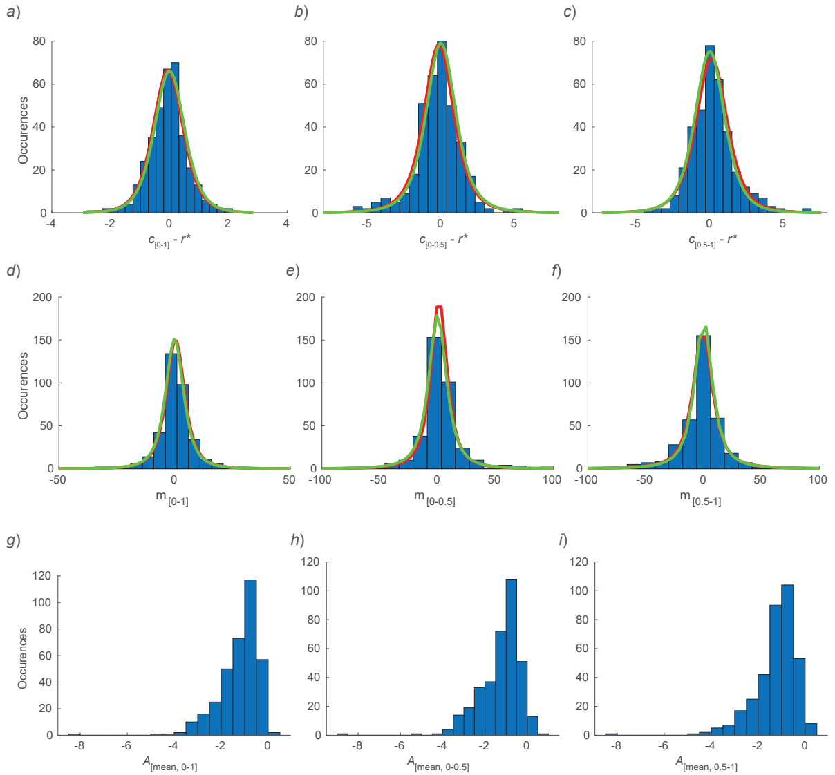
Figure S6: Distributions of nine parameters used in the constant- r extraction algorithm (related to Figures 4 – 6). (a) c_{[0-1]} - r^* , (b) c_{[0-0.5]} - r^* , (c) c_{[0.5-1]} - r^* , (d) m_{[0-1]} , (e) m_{[0-0.5]} , (f) m_{[0.5-1]} , (g) A_{[\text{mean}, 0-1]} , (h) A_{[\text{mean}, 0-0.5]} , and (i) A_{[\text{mean}, 0.5-1]} . In blue, histograms of nine parameters obtained from manual selection of 355 constant- r segments in 313 (out of first 532) landing manoeuvres for high light condition and spoke landing pattern. In red, estimated probability density functions of first six parameters (generalized student's t -distributions, see Table S8 for parameter values). In green, the representative probability density functions of first six parameters used in constant- r extraction algorithm (location parameter \mu for these six parameters is zero, scale parameter \sigma is \sigma_1, 2\sigma_1, 2\sigma_1, \sigma_2, 2\sigma_2 and 2\sigma_2 for panels (a)-(f), respectively (where \sigma_1 = 0.53 and \sigma_2 = 4.22 ) and shape parameter \nu is same as in Table S8).
