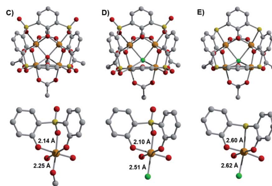
Fig. 2 Structure of (sc4a)Fe(btc) (A) and (tc4a)Fe(btc) (B) where orange, yellow, green, gray, and red spheres represent iron, sulfur, chlorine, carbon, and oxygen, respectively. Hydrogen atoms and charge-balancing cations are omitted for clarity. Although the structures of these cages are similar, the metal building units of (sc4a)Fe(btc) (D) and (tc4a)Fe(btc) (E) are significantly distorted as compared to (sc4a)Fe(OAc) (C).
