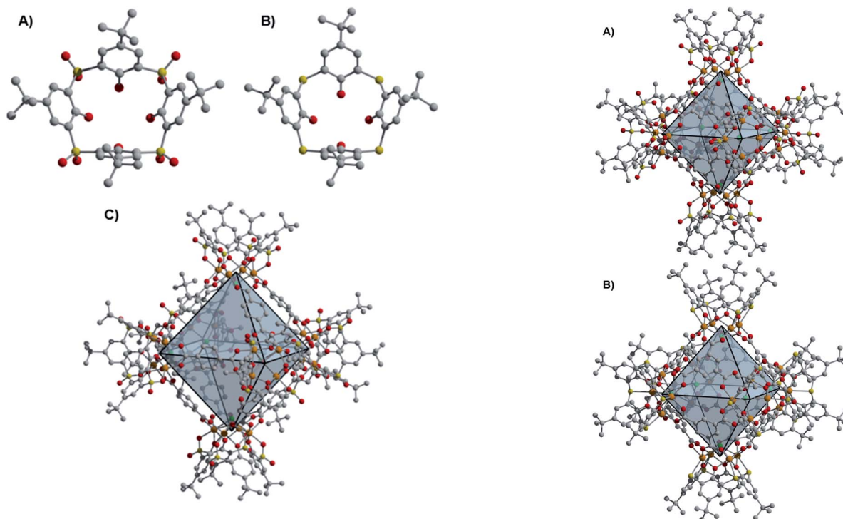
Fig. 1 Structures of the sulfonylcalix[4]arene (sc4a, (A)) and thiacalix[4]arene (tc4a, (B)) capping ligands, as well as [(\text{Fe}_{24}\text{Cl}_6(\text{sc4a})_6(\text{bdc})_{12})]^{6-} ((sc4a)Fe(bdc); (C)) where orange, yellow, green, gray, and red spheres represent iron, sulfur, chlorine, carbon, and oxygen, respectively. Hydrogen atoms and charge-balancing cations are omitted for clarity.
