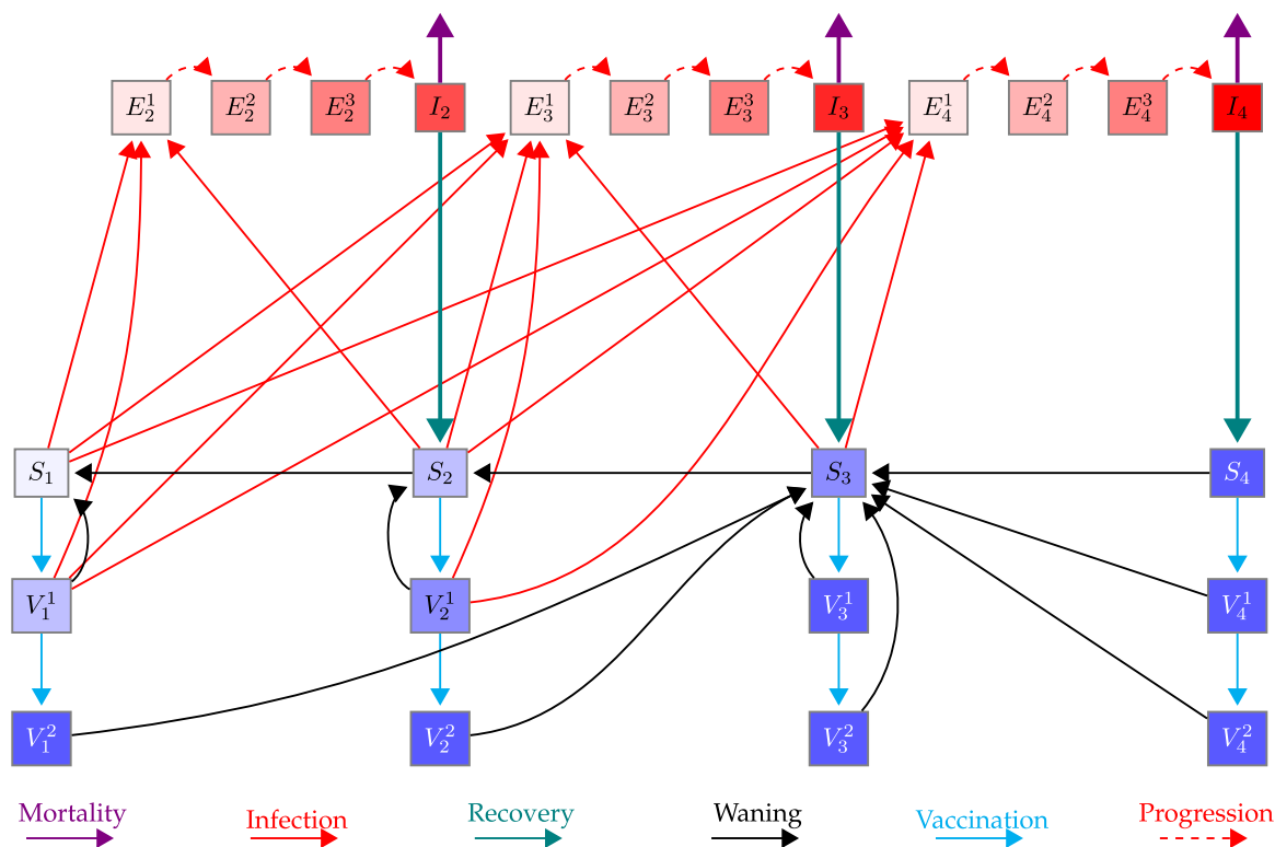
Fig. 1. Schematic of the model for one age group. Here, S_1 , S_2 , S_3 , and S_4 (purple shaded boxes) represent susceptible individuals who are immunologically naive, have some, moderate, and full immunity, respectively. I_2 , I_3 , and I_4 (red boxes) represent infected individuals with mild, moderate and severe symptoms, respectively, who will develop some, moderate, and full immunity once recovered (teal lines), respectively. E_i^k ( i = 2, 3, 4; k = 1, 2, 3 ) represent exposed individuals (infected, asymptomatic, not infectious) with progressive stages k = 1, 2, 3 that will experience mild I_2 , moderate I_3 , and severe I_4 symptoms. Susceptible and vaccinated individuals can be infected and move to the exposed classes (red lines). Susceptible and vaccinated classes at the same location on the immunity continuum have similar characteristics. Immunity gained from infection and vaccination can wane (black lines). (For interpretation of the references to color in this figure legend, the reader is referred to the web version of this article.)
