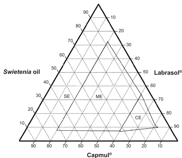
Figure 4 Ternary phase diagram of System 4. Abbreviations: CE, coarse emulsion; ME, macroemulsion; SE, separation emulsion.
