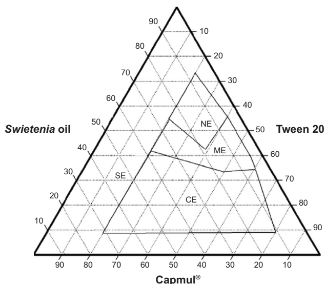
Figure 2 Ternary phase diagram of System 2. Abbreviations: CE, coarse emulsion; ME, macroemulsion; NE, nanoemulsion; SE, separation emulsion.
