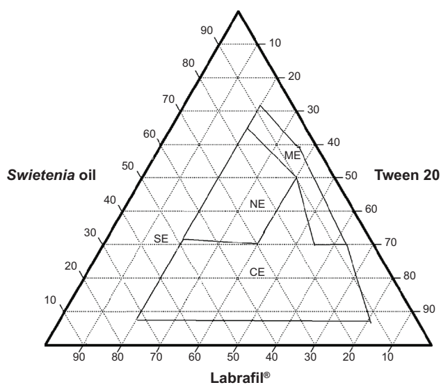
Figure 3 Ternary phase diagram of System 3. Abbreviations: CE, coarse emulsion; ME, macroemulsion; NE, nanoemulsion; SE, separation emulsion.
