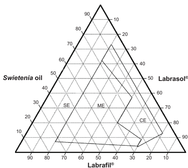
Figure 5 Ternary phase diagram of System 5. Abbreviations: CE, coarse emulsion; ME, macroemulsion; SE, separation emulsion.
