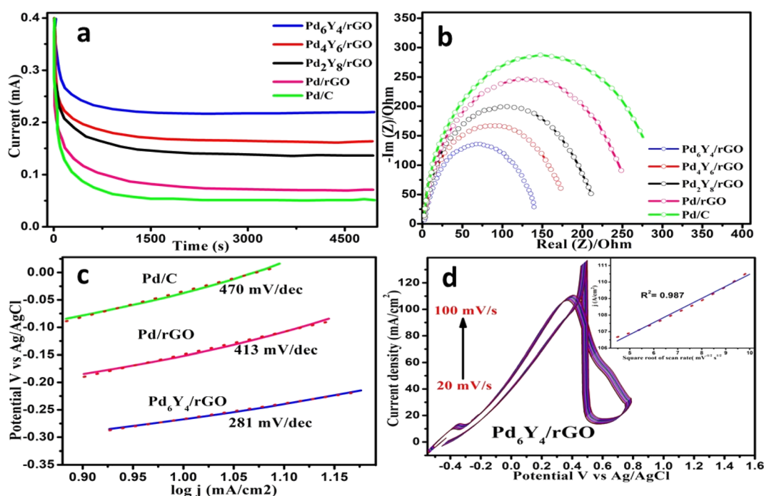
Fig. 3 (a) Current vs. time profile of \text{Pd}_x\text{Y}_y/\text{rGO} s and reference catalysts (b) Nyquist profile of \text{Pd}_x\text{Y}_y/\text{rGO} s and reference catalysts (c) Tafel slope of \text{Pd}_6\text{Y}_4/\text{rGO} and reference catalysts (d) transport characteristics of \text{Pd}_6\text{Y}_4/\text{rGO} .
