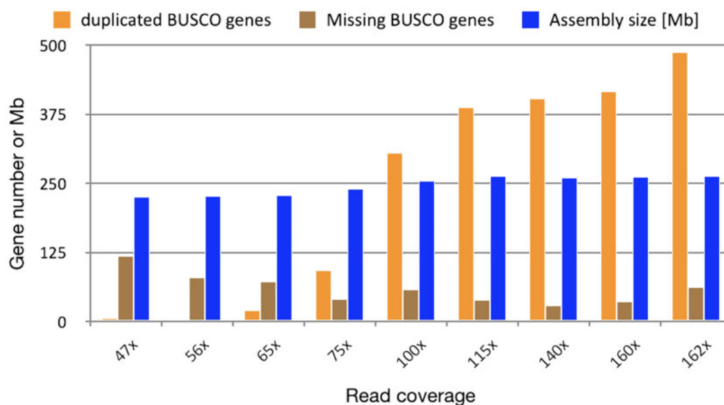
Figure 2 Raw read coverage effect on assembly size and quality. Please note that assembly size is provided in mega base pairs.
