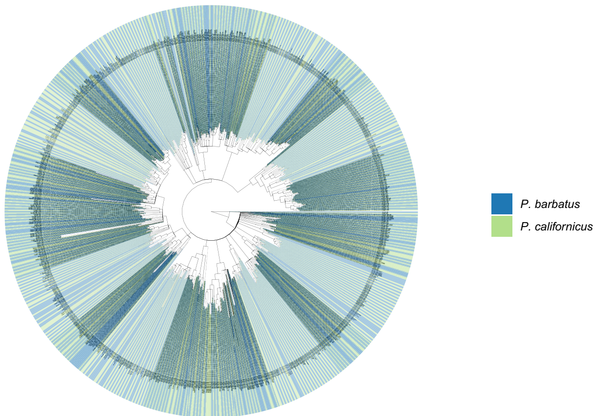
Figure 3 OR gene repertoires are similar between P. californicus (N = 417 genes) and P. barbatus (N = 453 genes). Most gene models have their closest relative in the other species. The gene tree shows no large clusters containing genes exclusively of one of the two species. This is evidence for a close relatedness between the species and an equally high quality of the two genome assemblies.
