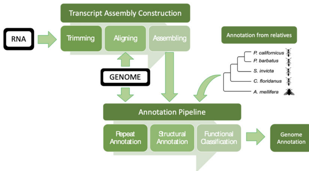
Figure 1 Overview of the annotation workflow. The workflow includes a construction of the transcript assembly (upper part) and a pipeline for the genome annotation (lower part). The transcript assembly and annotations from related species are providing evidence for the annotation of PCGs.
