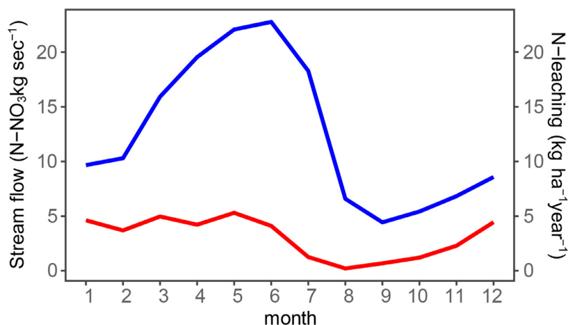
Fig. 5. Comparison of simulated N-leaching and reported N-NO 3 flow at the USGS Gage Station on the Mississippi River near Grafton, Illinois. Monthly flow of both sources was averaged across years.
