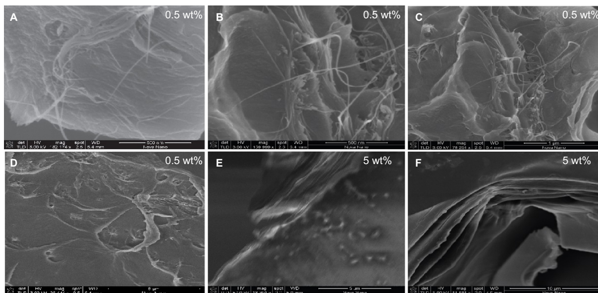
Figure 2 Scanning electron microscopy micrographs of the SWCNT/PMMA composites (A) 0.5 wt%–500 nm, (B) 0.5 wt%–500 nm, (C) 0.5 wt%–1 μm, (D) 0.5 wt%–5 μm, (E) 5 wt%–5 μm, and (F) 5 wt%–10 μm.
