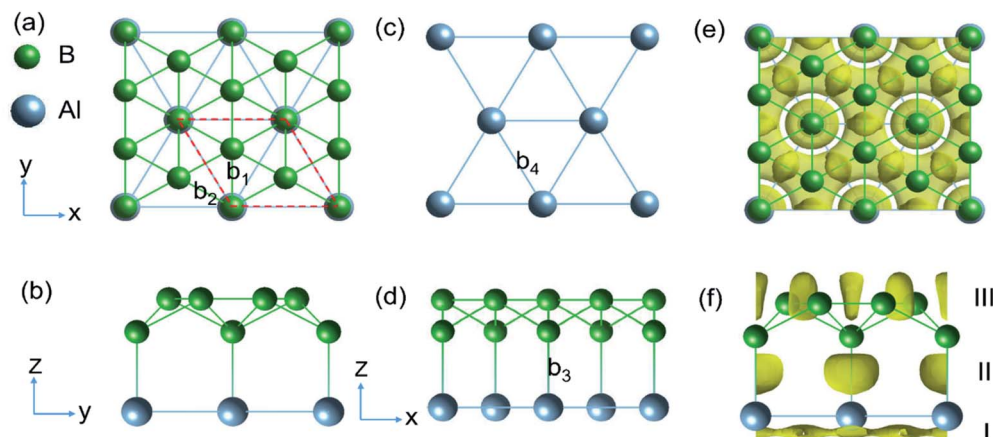
Fig. 1 (a, b and d) Top and side view of the AlB_3 heterosheet. The red dashed lines in (a) represent the primitive cell of the layer. (c) Al (111) sublayer. (e and f) Corresponding electron localization function (ELF) with an isovalue of 0.75. Three ELF domains are marked by Roman numerals in (f) and discussed in the text.
