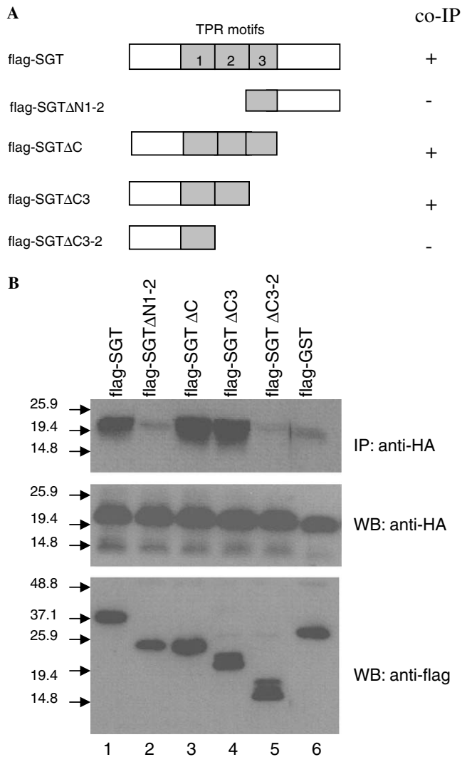
Fig. 4. TPR2 is essential for the interaction with SARS-CoV 7a-HA. (A) Full-length flag-hSGT (aa 1-313) and deletion mutants flag-hSGTΔN1-2 (aa 159-313), flag-hSGTΔC (aa 1-192), flag-hSGTΔC-3 (aa 1-158), and flag-hSGTΔC3-2 (aa 1-125) are shown. All hSGT proteins were flag-tagged at the N-terminus. The locations of the TPR motifs 1, 2, and 3 are represented by shaded boxes. The name of each clone is shown on the left and results of the co-IP are shown on the right. (B) Flag-tagged full-length or mutant hSGT were co-transfected into Vero-E6 cells with 7a-HA, respectively. Total proteins were extracted and co-immunoprecipitated with mouse anti-flag beads. IP complexes (upper panel) and total cell lysates (middle and lower panel) were Western blotted and probed with rabbit anti-flag or rabbit anti-HA antibodies.
