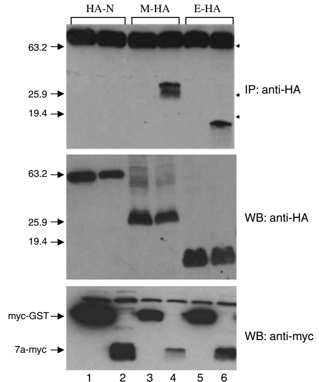
Fig. 5. 7a-myc interacts with SARS-CoV structural proteins. Total cell lysates from cells co-transfected with myc-GST or 7a-myc with either HA-N, E-HA or M-HA were immunoprecipitated with myc-polyclonal antibody conjugated to Protein A-beads. IP complexes (upper panel) and total cell lysates (middle and lower panel) were Western blotted and probed with mouse anti-myc or mouse anti-HA antibodies.
