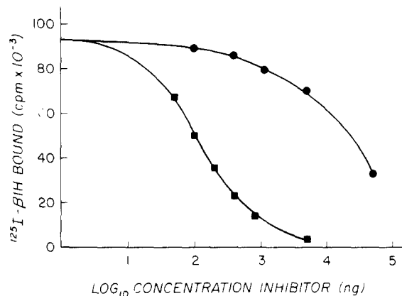
FIG. 5. Inhibition of ^{125}\text{I} - \beta 1H binding to EAC14 oxs 23 by unlabeled \beta 1H (■) or B (●).
