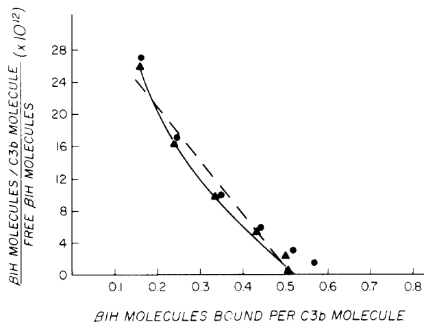
FIG. 4. Scatchard analysis of binding of ^{125} I- \beta 1H to EAC14 ox 23 prepared with ^{131} I-C3. The latter allowed the enumeration of the numbers of C3b molecules which was 64,000/cell for this experiment. As in Fig. 4, total binding (●) and that corrected for EAC14 ox 2 (▲) binding are given. The dashed and smooth lines are also the same as in Fig. 3.
