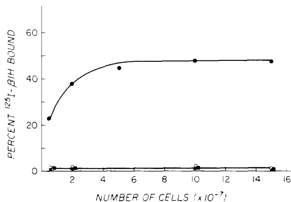
FIG. 2. Percent of ^{125}\text{I} - \beta 1H bound by varying numbers of EA (▲), EAC14 (○), EAC14 ox 2 (■) or EAC14 ox 23 (●).
