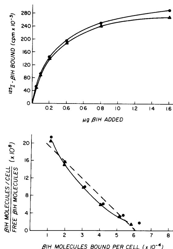
FIG. 3. Quantitative analysis of the interaction of varying concentrations of ^{125}\text{I}-\beta 1\text{H} with \text{EAC14}^{\text{oxy}23} . In the upper panel the cpm ^{125}\text{I}-\beta 1\text{H} bound is shown as a function of the amount of ^{125}\text{I}-\beta 1\text{H} added; the lower panel is a Scatchard analysis of the same data (see text). In both, total binding to \text{EAC14}^{\text{oxy}23} (●) and binding corrected for \text{EAC14}^{\text{oxy}2} (▲) are shown. In the lower panel the dashed straight line has been fit by the method of least squares to the corrected data, and the unbroken line is a smooth curve drawn by hand through the same points.
