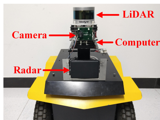
Figure 8. The wheeled robot used in our experiments, equipped with a LiDAR, a mmW-radar, a camera and a computer.
