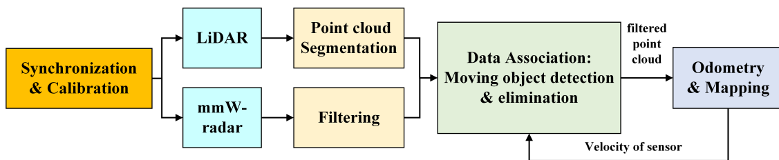
Figure 4. The system overview of moving objects elimination.
