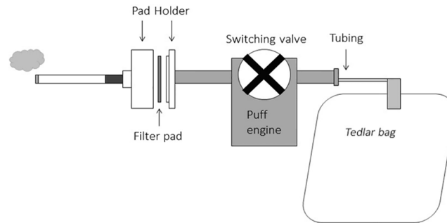
Fig 1. Pad + Bag mainstream smoke collection diagram.
