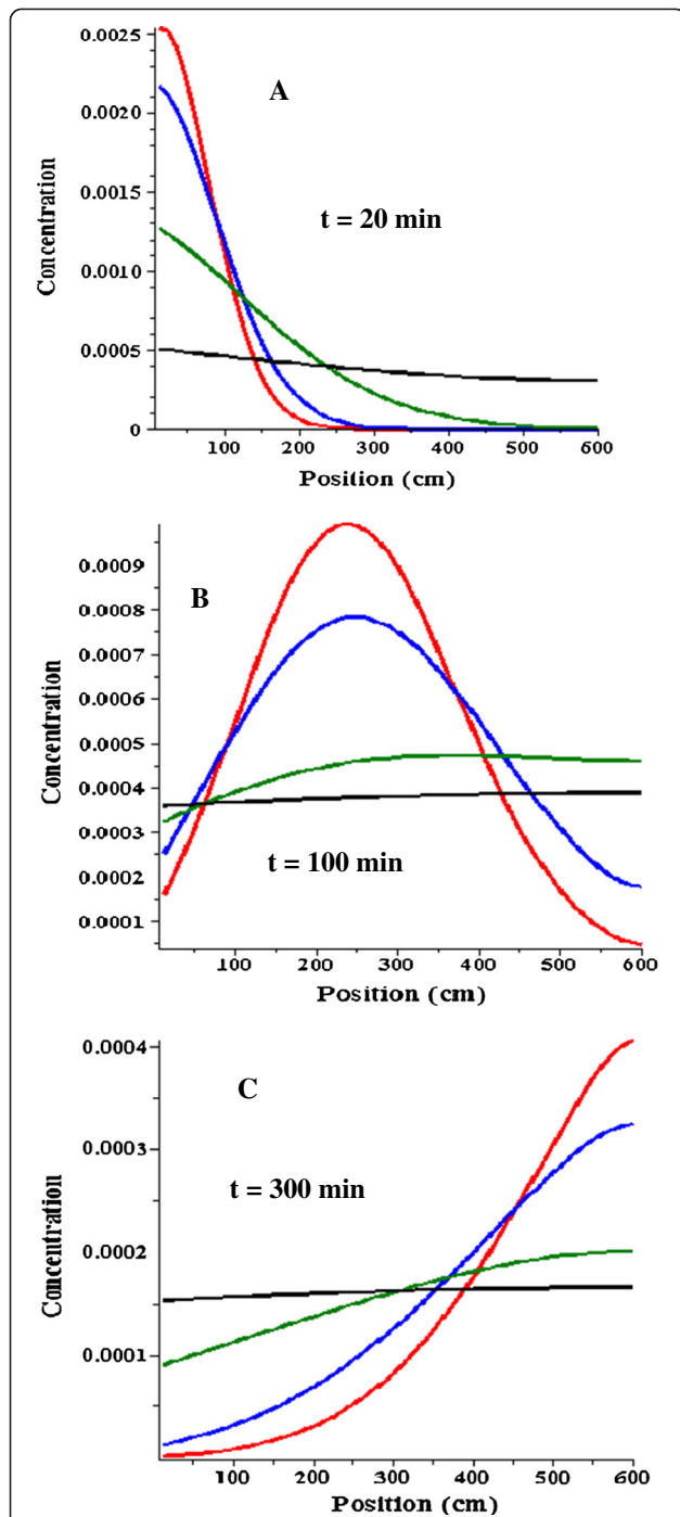
Figure 5 Diffusion convection concentration profile. The diffusion convection model concentration as a function of distance from the pyloric sphincter is shown at 20 (Figure 5A), 100 (B) and 300 minutes (C) after administering the oral dose as a bolus to the stomach for an impermeable ( P = 0 ) solute. The profile is shown for 4 different values of the dispersion time constant ( T_D ): 2000 (red); 1000 (blue); 200 (green); and 20 minutes (black). For all profiles T_F = 200 minutes; T_G = 15 minutes; r = 1 cm; L = 600 cm and Dose = 1.
