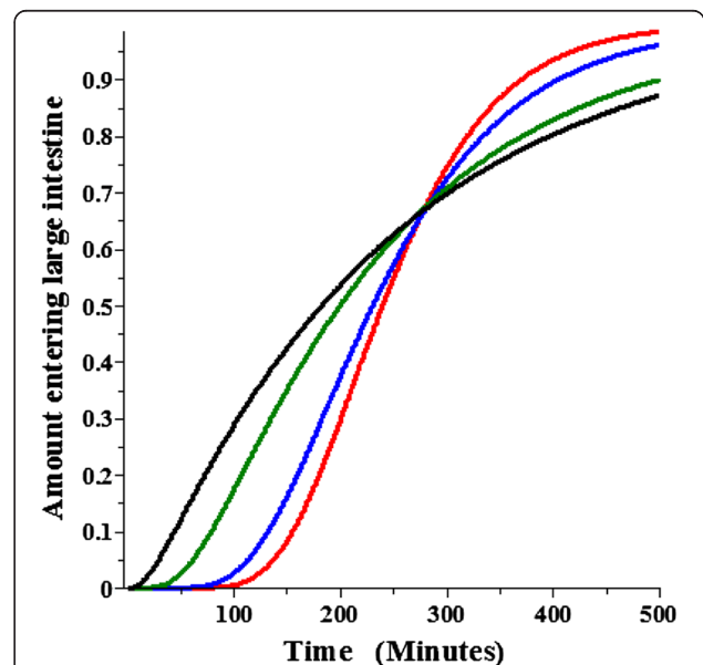
Figure 6 Diffusion convection small intestinal transit time. The diffusion convection amount leaving the small intestine and entering the large intestine as a function of time for an impermeable solute. Same conditions as for Figure 5.
