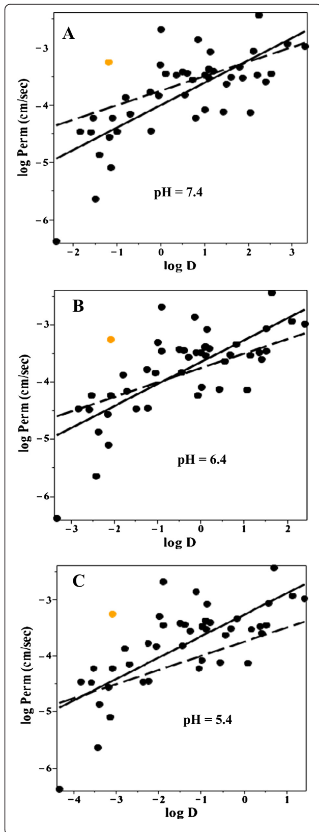
Figure 11 Permeability versus octanol partition for basic solutes. Plot of the log of the permeability (cm/sec) versus the log of the octanol/water partition (log D) for the basic solutes in Additional file 1: Table 2. The log D was determined at pH = 7.4 (Figure 11A), 6.4 (Figure 11B) and 5.4 (Figure 11C). The solid line is the linear regression fit to the black points and the dashed line is the linear regression fit to the neutral solutes (Figure 10). The orange point is midodrine which is a substrate for the peptide transport system.
