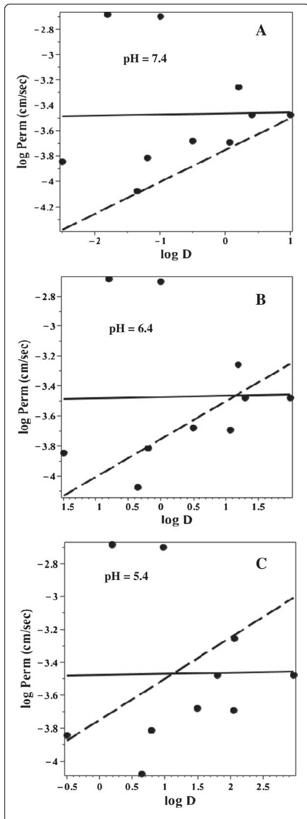
Figure 12 Permeability versus octanol partition for acidic solutes. Plot of the log of the permeability (cm/sec) versus the log of the octanol/water partition (log D) for the acidic solutes in Additional file 1: Table 2. The log D was determined at pH = 7.4 (Figure 12A), 6.4 (Figure 12B) and 5.4 (Figure 12C). The solid line is the linear regression fit to the black points and the dashed line is the linear regression fit to the neutral solutes (Figure 10).
