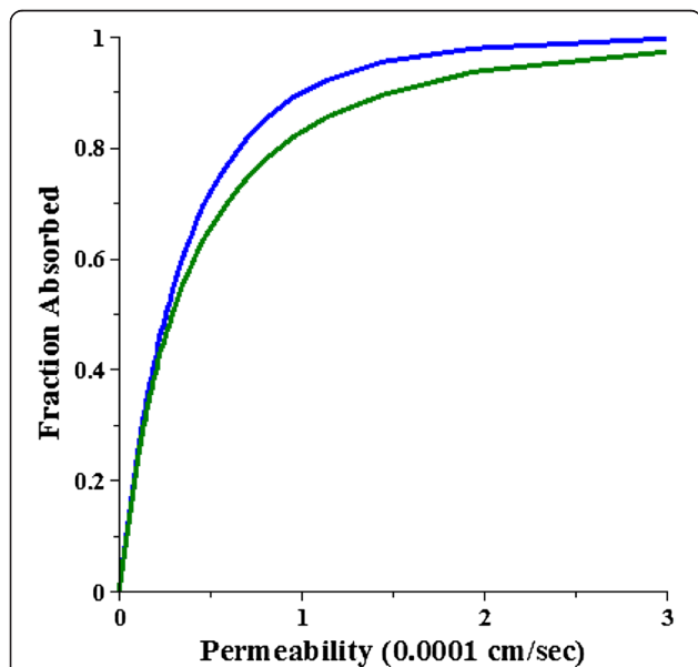
Figure 7 Permeability dependence of the diffusion convection intestinal absorption. The fractional absorption of the diffusion convection model as a function of the permeability in units of 10^{-4} cm/sec for a dispersion time constant ( T_D ) of 1000 (blue) or 200 minutes (green). The rest of the conditions are the same as in Figure 5.
