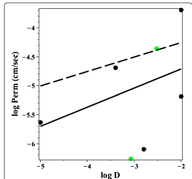
Figure 13 Permeability versus octanol partition for charged solutes. Plot of the log of the permeability (cm/sec) versus the log of the octanol/water partition (log D) for the charged solutes in Additional file 1: Table 2. The solid line is the linear regression fit to the black points and the dashed line is the linear regression fit to the neutral solutes (Figure 10). The green points are cefixime and aztreonam which are substrate for the P-glycoprotein mediated efflux system.
