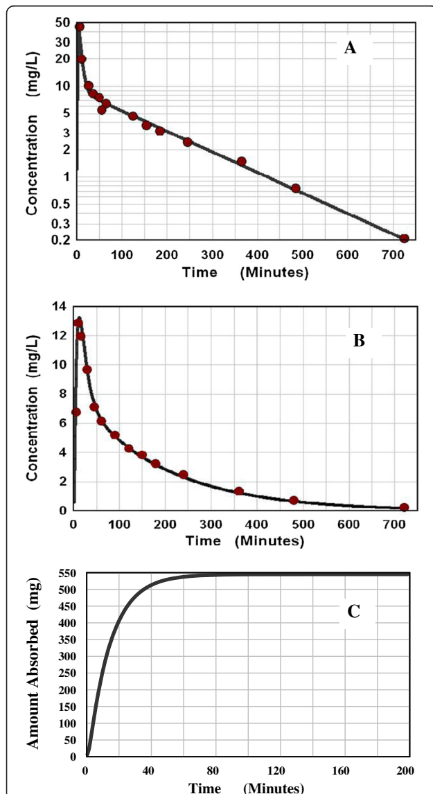
Figure 1 AM model deconvolution solution for intestinal absorption of acetaminophen. Figure 1A shows a comparison of the experimental blood concentration data points (red circles) following an IV input versus the theoretical blood concentration determined from the 2 exponential systemic response function (line). Figure 1B shows a comparison of the experimental blood concentration data points (red circles) following an oral input with the theoretical blood concentration prediction determined from the deconvolution solution of the AM absorption rate function. Figure 1C shows the cumulative AM absorption amount as a function of time.
