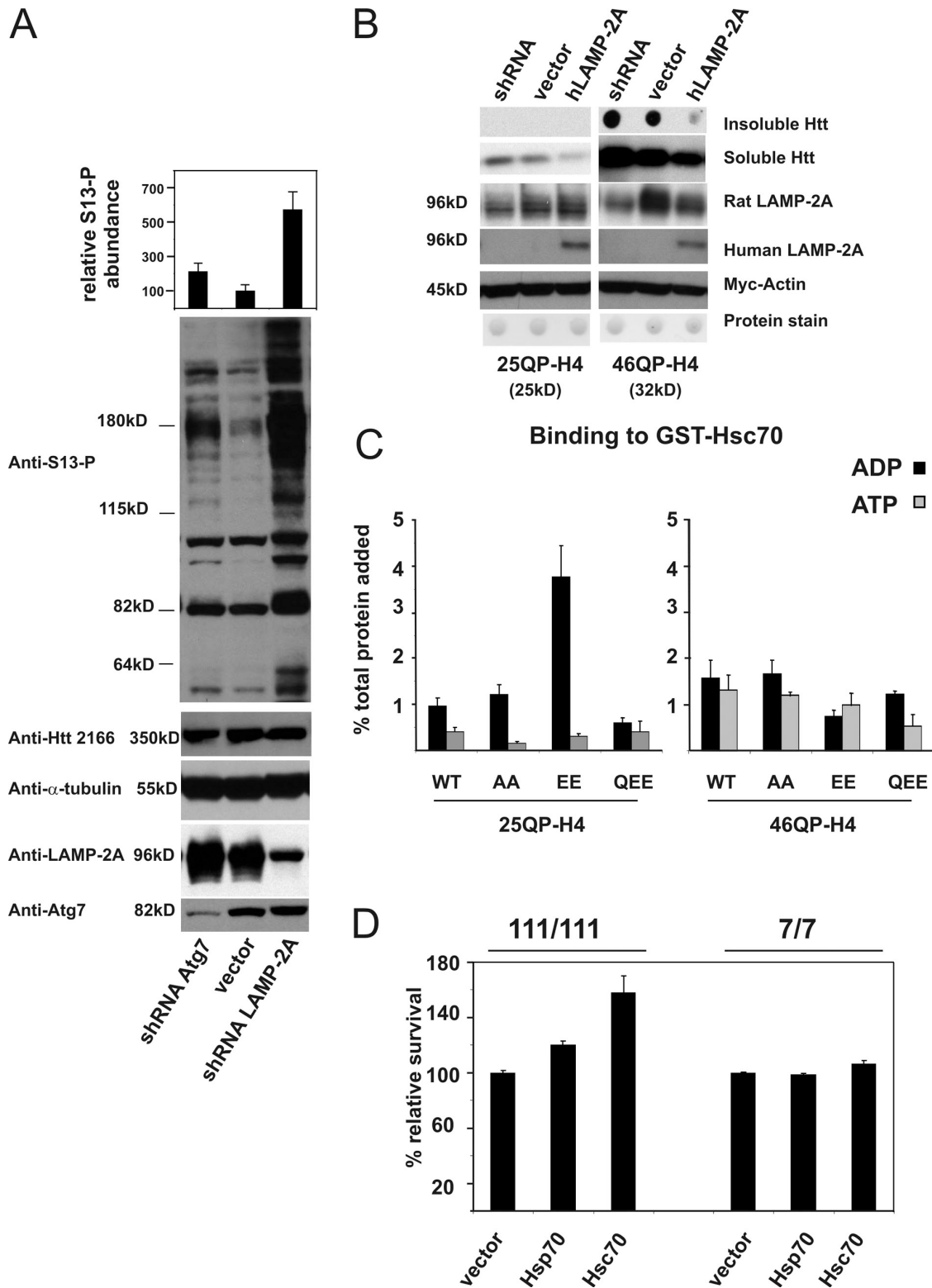
Figure 6. LAMP-2A, Atg7, and Hsc70 may modulate Htt clearance and toxicity. (A) Reducing levels of LAMP-2A or Atg7 in cell culture increases abundance of S13-phosphorylated Htt. Si14A cells were transiently transfected with shRNA for rat LAMP-2A or Atg7, or pSUPER vector control; antibodies used for Western analysis are shown to the left of the Western panels. (B) LAMP-2A levels modulate Httex1p abundance. Si14A cells were transiently cotransfected with LAMP-2A shRNA, human HA-tagged LAMP-2A or vector control, and myc-actin transfection control. Lysates were subjected to Western analysis and filter-retardation assay, detected with anti-Htt CAG53b, anti-rat/mouse LAMP-2A, anti-HA to detect HA-hLAMP-2A, anti-myc, and MemCode protein stain. (C) Hsc70 interacts with phosphomimetic unexpanded polyQ Httex1p in vitro. Purified 25QP-H4 or 46QP-H4 wt and mutant proteins radiolabeled with ^{35}\text{S} were incubated with isolated GST-Hsc70 or GST protein bound to glutathione-agarose beads. Where indicated, 5 mM ATP or ADP was added to the reaction. Bound proteins were washed, subjected to SDS-PAGE, and detected by phosphoimager autoradiography. (D) Hsc70 reduces Htt-mediated toxicity in Hdh 111/111 cells. Hdh 7/7 or Hdh 111/111 cells were nucleofected with vector, Hsp70, or Hsc70 together with GFP. 47 h later, XTT cell viability assays were performed, and the percentage of relative survival was calculated correcting for transfection efficiency of the GFP control \pm SEM from triplicates.
