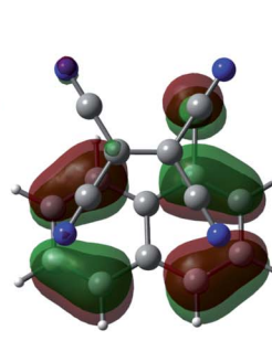
Fig. 1 TCNE: \pi :1CIN CT complex (left) and top view of frontier molecular orbitals (isovalue: 0.03) mainly involved in the S_1 \leftarrow S_0 and S_2 \leftarrow S_0 electronic transitions. From left to right, HOMO-1, HOMO and LUMO contour plots computed for a minimum energy structure in DCM solvent. Carbons are reported in gray, hydrogens in white, blue is for nitrogens and green for chlorine atoms.
