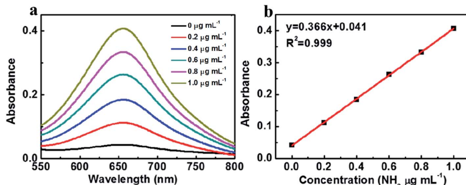
Fig. 3 (a) UV-vis absorption spectra of different concentration ammonia in 0.1 M \text{Na}_2\text{SO}_4 solution, (b) standard curve of ammonia in 0.1 M \text{Na}_2\text{SO}_4 solution.
