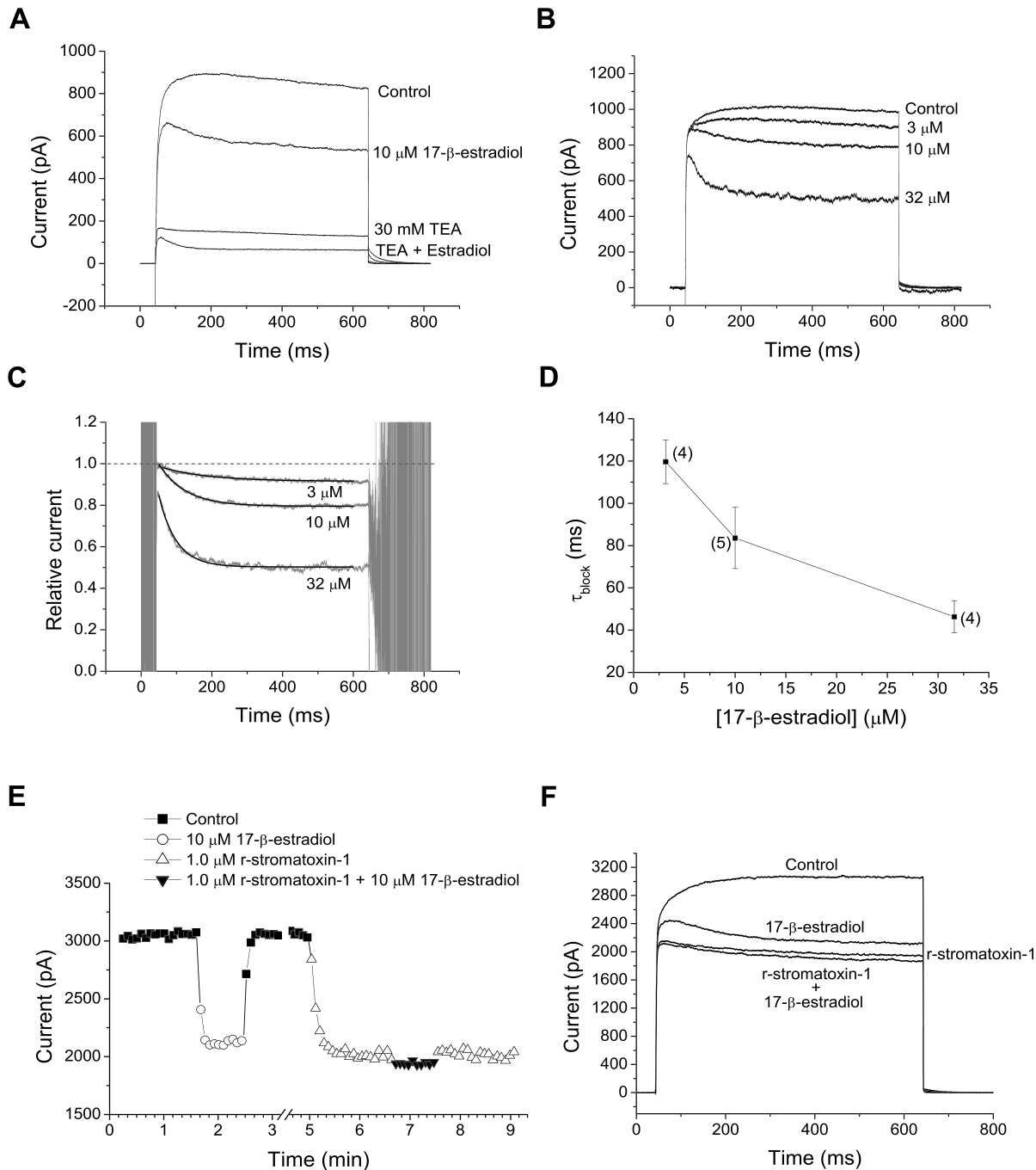
Figure 3. Sensitivity to blockers and concentration-dependent rate of current decline. A, currents (averages of 10 traces) evoked by a voltage step from -74 mV to +6 mV in solutions as indicated. Note that 30 mM TEA blocked a major fraction of the voltage-activated K + current without leaving any significant transient current remaining. Note also that the blocking effects of TEA and 17- \beta -estradiol were overlapping. B, currents evoked by voltage steps from -74 mV to +26 mV, in control solution and in the indicated concentrations of 17- \beta -estradiol. Note the faster current decline and the larger block with increasing concentration of 17- \beta -estradiol. C, ratio of current (grey) in 17- \beta -estradiol to that in control solution, to show the time course of current inhibition. The traces were well fitted by exponential functions with time constants 134ms (top), 75ms (middle) and 49 ms (bottom), shown as superimposed black lines. Computed from the traces shown in B. D, dependence of time constant of relative current, as in C, on concentration of 17- \beta -estradiol. Mean \pm S.E.M. for the number of neurons indicated. Voltage steps to +26 mV from -74 mV. E-F, overlapping block by estradiol and r-stromatoxin-1. E, time-course of block of the K + current (mean current 590–600 ms after a voltage step from -74 to +26 mV) by estradiol, r-stromatoxin-1 and a combination of these substances, as indicated. F, K + currents (averages of 10 traces) evoked by voltage steps from -74 to +26 mV. Concentration of blockers as in E. Note the lack of effect of estradiol in the presence of r-stromatoxin-1. Data in E and F from the same neuron.
