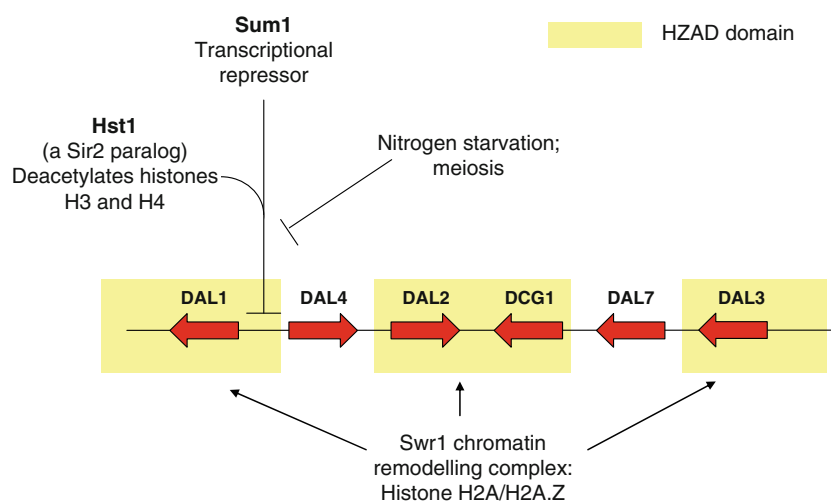
Fig. 6 Activation of expression of the DAL genes. The DAL gene cluster lies within an HZAD domain, in which histone H2A is replaced by the histone variant H2A.Z (Htz1) [83]. H2A.Z protects euchromatin from the ectopic spread of silent heterochromatin (the region of Sir2-effected silencing closer to the telomere), and is present in (and enables expression of) the DAL1 , DAL2 , DCG1 and DAL3 genes but not DAL4 or DAL7 . Interestingly, while DAL1 ,
