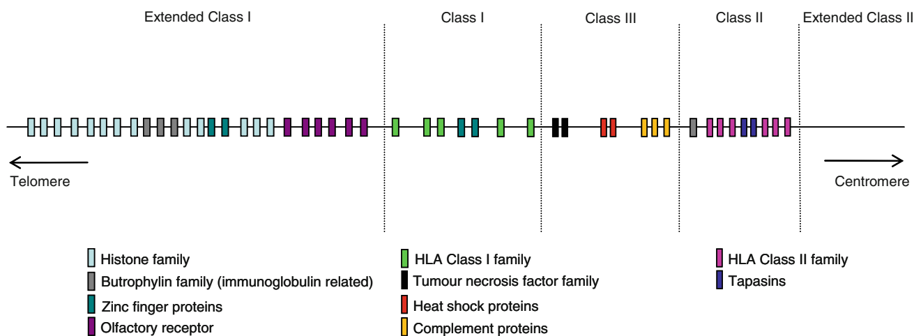
Fig. 8 The human major histocompatibility complex (MHC). A representation of the distribution of genes from large or immunologically important gene families across the ~7.5 Mb extended MHC on the short arm of human chromosome 6. Each coloured block
