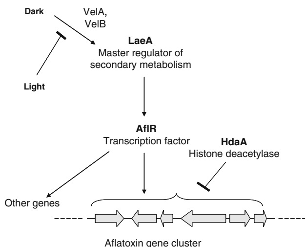
Fig. 3 Different levels of regulation of the aflatoxin gene cluster in the fungus, Aspergillus nidulans . The genes for aflatoxin biosynthesis are clustered in a 70-kb region and encode at least 23 co-regulated transcripts (not all cluster genes are shown in this diagram). The positive regulatory gene aflR lies within the gene cluster and is required for the transcriptional activation of most, if not all, pathway genes. aflR also regulates three genes outside the aflatoxin gene cluster. LaeA is a master regulator of secondary metabolism in the Aspergilli and is required for AflR -mediated expression of the aflatoxin biosynthetic cluster. LaeA also controls transcription of gene clusters for other secondary metabolites and is believed to act via chromatin remodeling. Histone deacetylase ( HdaA ) performs an opposing role to LaeA and functions to repress gene expression in this region. Synthesis of secondary metabolites in the Aspergilli is linked to environmental stimuli and development. In the light asexual development (sporulation) is induced and genes involved in aflatoxin are not expressed. Darkness induces sexual development with associated induction of metabolite production, mediated by the proteins VelB and VeA . Adapted from [33]
