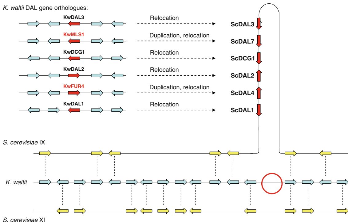
Fig. 5 The birth of the DAL gene cluster. The DAL gene cluster on S. cerevisiae chromosome IX (red) lies within a sister region between chromosomes IX and XI (genes shown in pale yellow). The corresponding region in K. waltii , a yeast species that does not contain the DAL gene cluster, contains a merge from these two chromosomes (genes shown at the bottom in pale blue). The K. waltii
