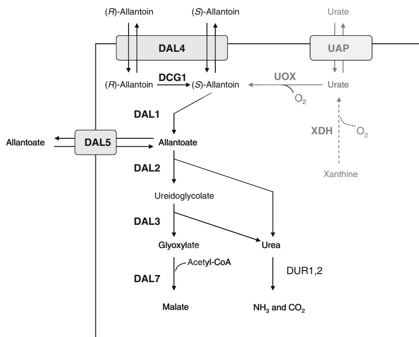
Fig. 4 The allantoin degradation pathway—an adaptation to growth under oxygen-limiting conditions in Saccharomyces cerevisiae . In the classical purine degradation pathway, xanthine is converted to urate and then to allantoin, in two successive oxidation steps catalyzed by the peroxisomal enzymes xanthine dehydrogenase (XDH) and urate oxidase (UOX). XDH genes are present in filamentous fungi but not in yeasts. To use purine derivatives as a nitrogen source yeasts must therefore import urate, allantoin or allantoate from outside the cell. Yeasts that lack the DAL cluster (e.g., Kluyveromyces lactis , Saccharomyces kluyveri , and Zygosaccharomyces rouxii ) are all able to grow on urate as a sole nitrogen source, presumably using urate permease (UAP) to import it, UOX to oxidize it and the DAL pathway enzymes to break it down to urea. In contrast, S. cerevisiae and Saccharomyces castellii have lost the ability to use urate, have no UOX or UAP genes, and instead import allantoin. The allantoin permease gene DAL4 is a duplicate of the uracil permease gene
