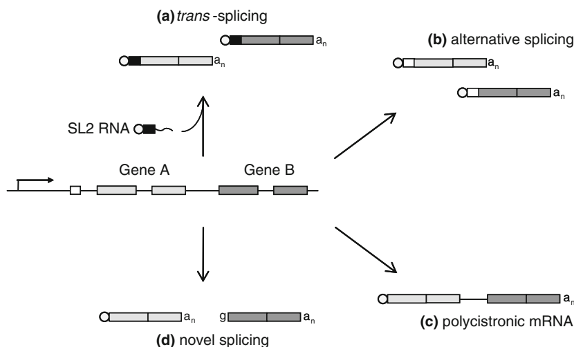
Fig. 11 Different strategies for the processing of eukaryotic operons. a The operons of Caenorhabditis elegans produce a polycistronic pre-mRNA that is processed into two or more mature monocistronic mRNAs by the trans -splicing machinery. The spliced leader sequence (black box) is derived from a spliced leader (SL) RNA which carries the 5' RNA cap (circle) [156]. b Alternative splicing of a polycistronic pre-mRNA can produce two mature mRNAs with a common first exon (white box) as observed at the conserved cholinergic locus [185]. c In some cases, such as for the Drosophila stoned locus,
