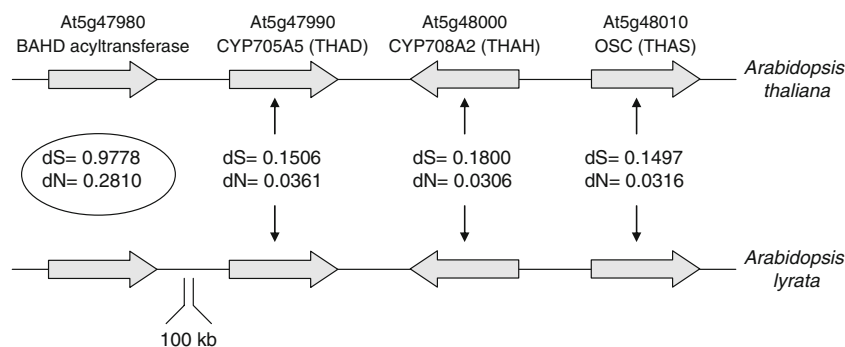
Fig. 7 The thalianol gene cluster in Arabidopsis . The A. thaliana gene cluster consists of four contiguous co-expressed genes encoding an oxidosqualene cyclase (THAS), two different types of cytochrome P450 (THAH and THAD) and a BAHD acyltransferase [101]. The organization of the equivalent region from the related crucifer,
